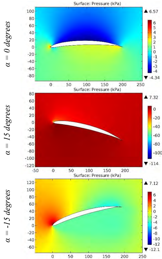
Figure 124. The pressure contours on the surfaces of the GOE 804 (EA 8) airfoil.
