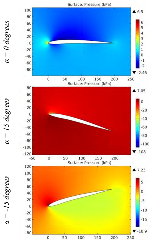
Figure 145. The pressure contours on the surfaces of the GRANTX16 airfoil.
