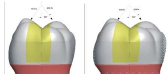
Figure 2 (a,b)- 3D Model and Load Application
