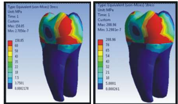
Figure 3: Von-Mises Stress distribution on restoration when tooth restored with GIC(Fuji IX)at (a) 450 N & (b) 600 N Load was applied.
