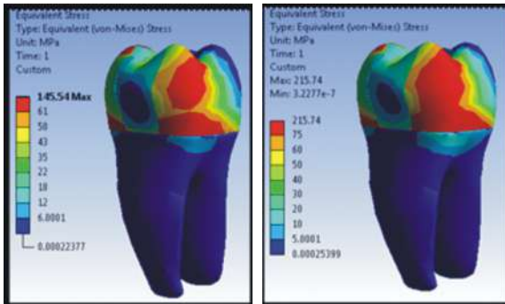
Figure 5: Von-Mises Stress distribution on restoration when tooth restored with Zirconomer at (a) 450 N and (b) 600 N Load was applied
