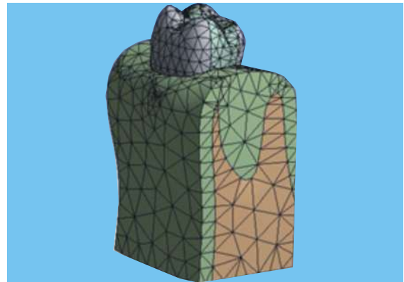
Figure 1: Model after Meshing
