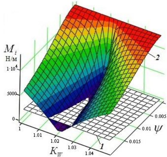
Fig. 6. Dependency graphs M_i = f(\psi, K_w) : 1 - M_Z = f(\psi, K_w) , 2 - M_Z = f(\psi, K_w)
