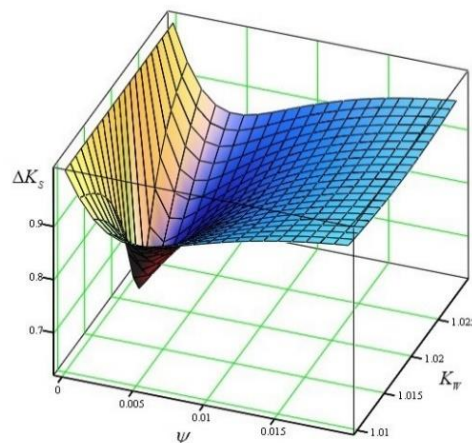
Fig. 3. Dependence graph \Delta K_N = f(\psi, K_W)
