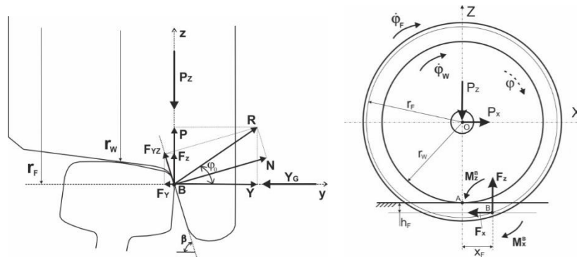
Fig. 1. Distribution of forces in the contact of a flange and a rail head at the moment of climbing: front view (left), side view (right)
