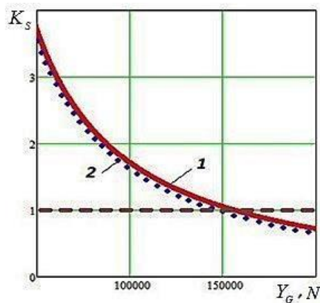
Fig. 2. The waveform of the safety coefficient K_S = f(Y_G) : 1 – the TWD of a wheel, 2 – the PWD type of a wheel
