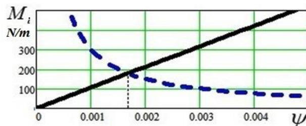
Fig. 5. Detail of the graph depicted in Figure 4
