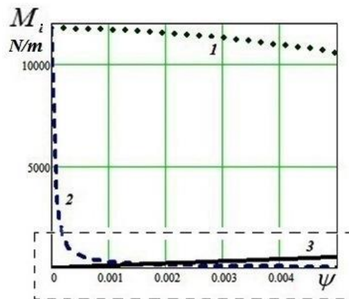
Fig. 4. Graph depicting the dependency of the values of M_i = f(\psi) : 1 - M_{X1} = f(\psi) (TWD type of wheel), 2 - M_{X2} = f(\psi) (PWD type of wheel), 3 - M_Z = f(\psi)
