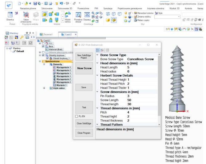
Fig. 5. Control application for generating CAD projects with a list of input parameters
