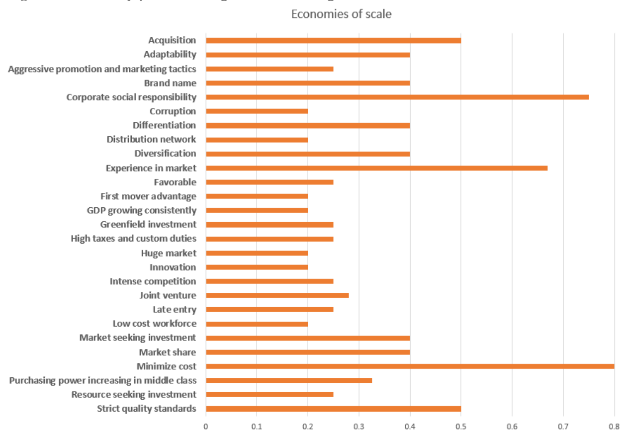
Figure 4: Proximity plot of economy of scale as the target item
