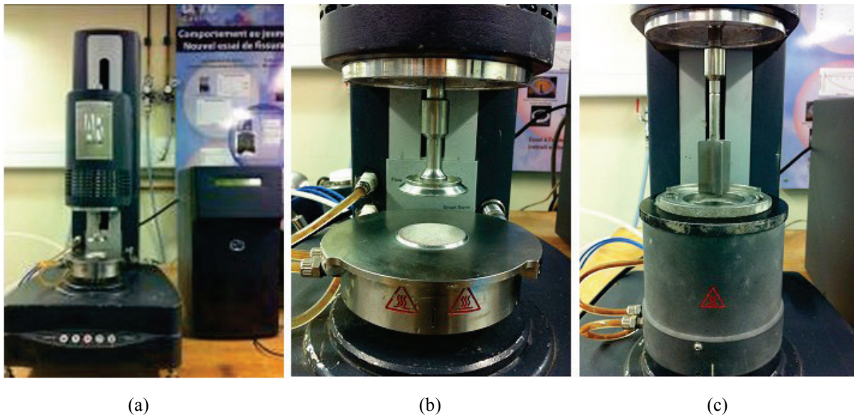
Figure 2: (a) Rheometer AR 2000, (b) parallel plates and (c) vane and cylinder
