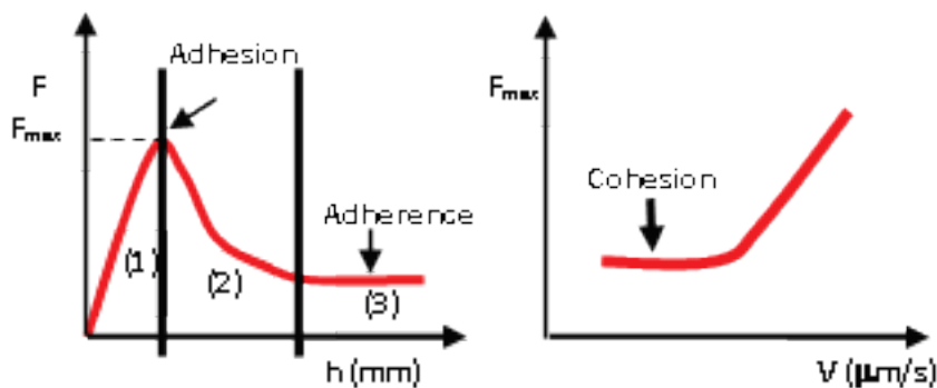
Fig. 1: Analysis of the tack test results. (a) General shape of the tack force curves; (b) evolution of the force peak versus stretching velocity.
