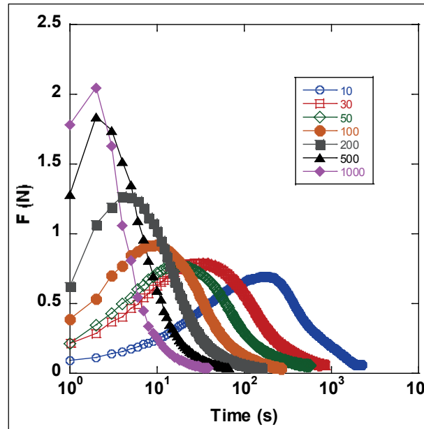
Fig. 6: Evolution of the stretching force versus time for different velocities (in \mu\text{m/s} ) for the 0.22% polymer paste.
