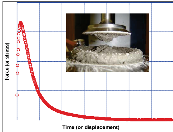
Fig. 7: Tack curve. Determination F and W
