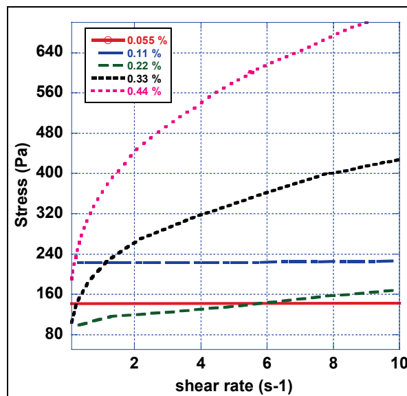
Fig. 5: Flow curves of the mortars for different polymer concentrations.
