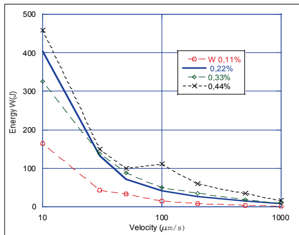
Fig. 8: Evolution of the energy needed to pull versus the velocity for different polymer concentrations
