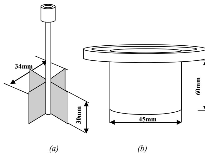
Fig.4: Rheological measurement system: a) vane, b) inner cylinder
