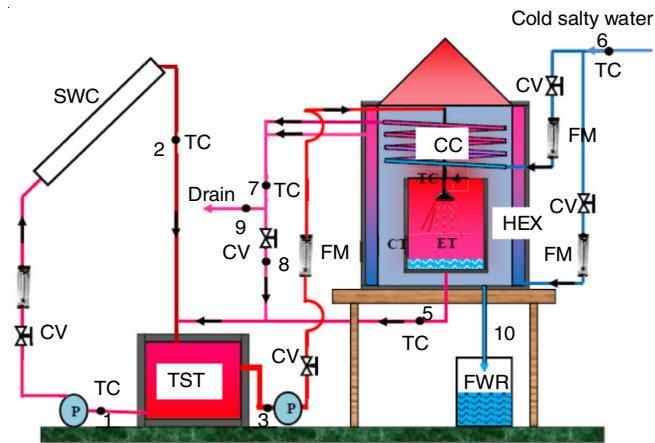
Fig. 12. Schematic view of the solar water desalination unit [Ref. 33]
