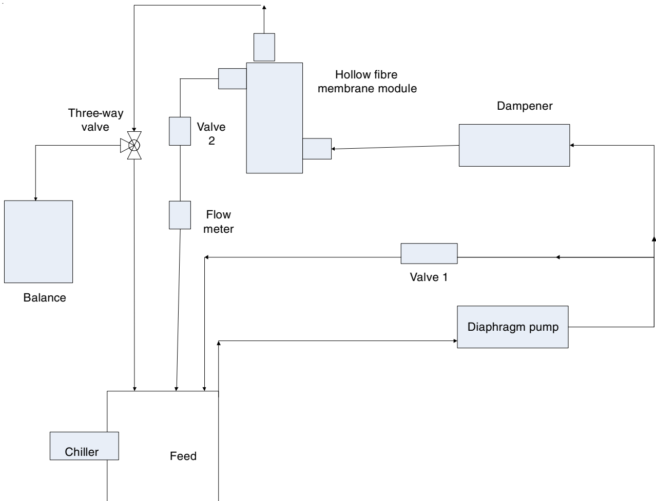
Fig. 10. Schematic diagram of the experimental nanofiltration set-up [Ref. 21]
