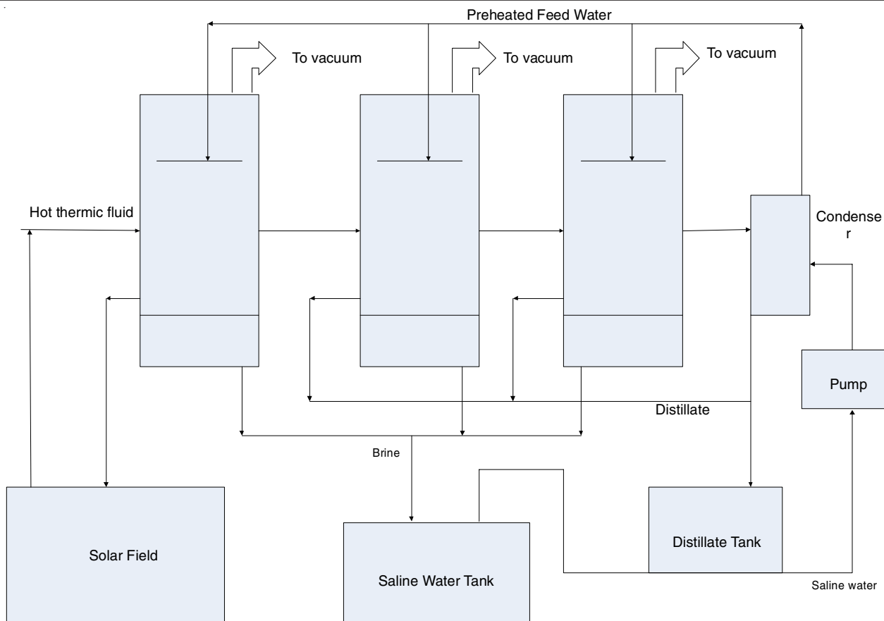
Fig. 5. Solar powered multi-effect distillation system [Ref. 7]
