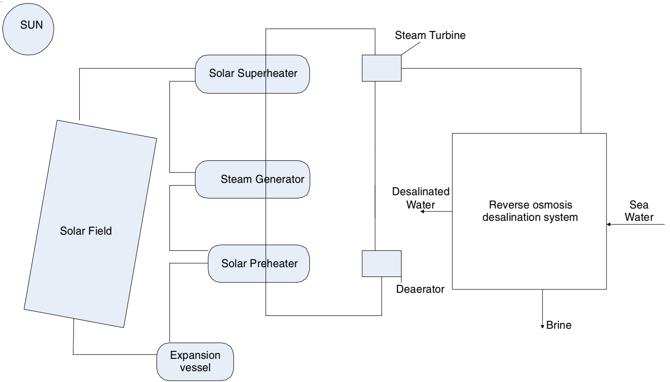
Fig. 9. Parabolic trough coupled with seawater reverse osmosis desalination unit [Ref. 4]
