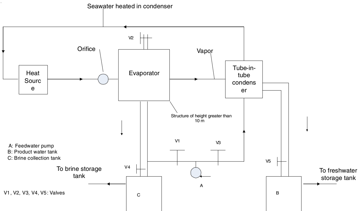
Fig. 4. Single-stage flash desalination system [Ref. 8]
