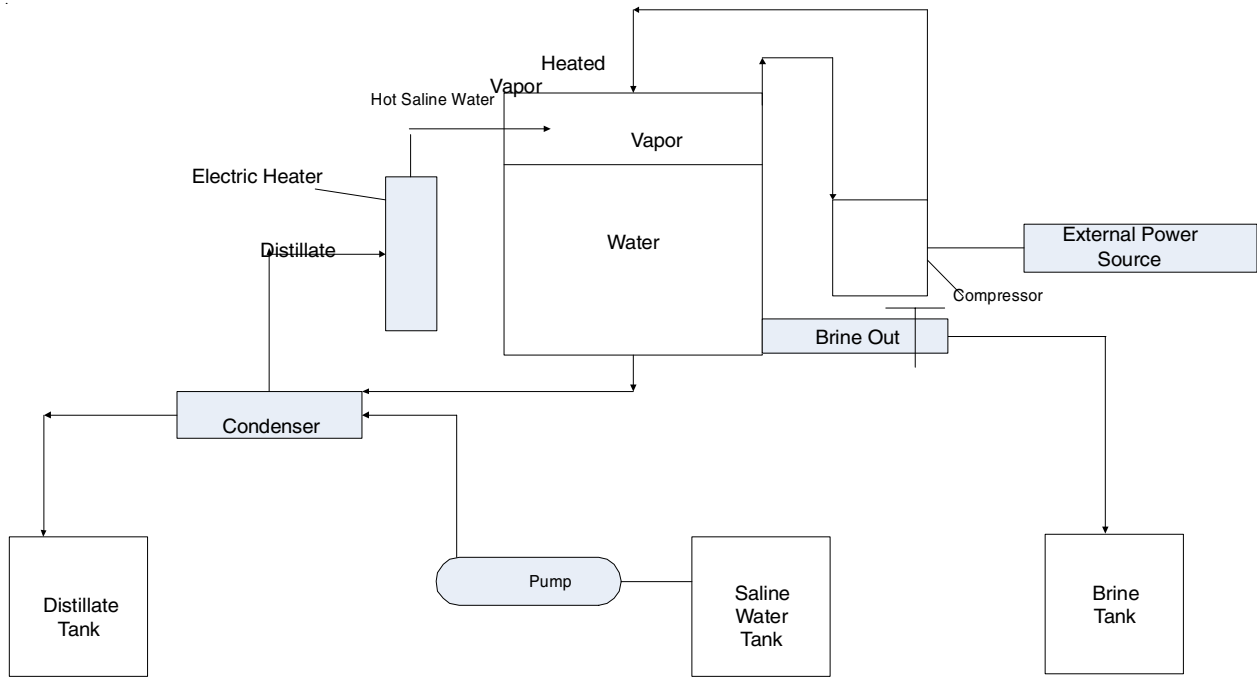
Fig. 6. Mechanical vapor compression desalination system [Ref. 7]
