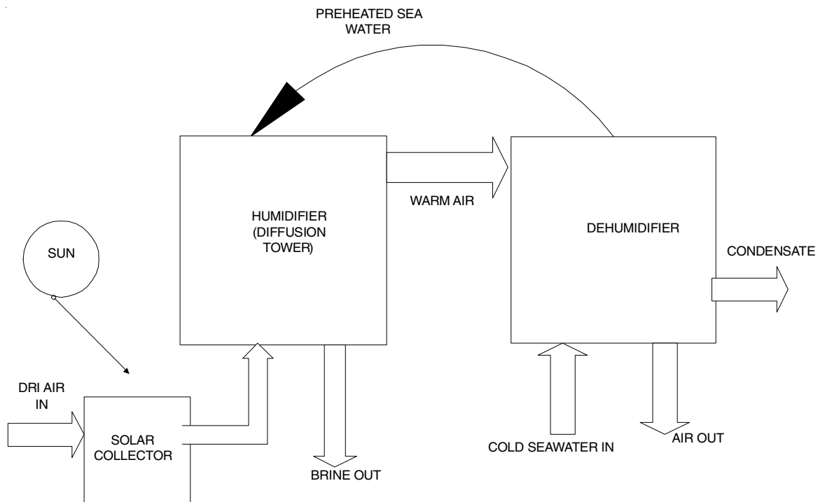
Fig. 7. A simple humidification–dehumidification (HDH) process [Ref. 16]
