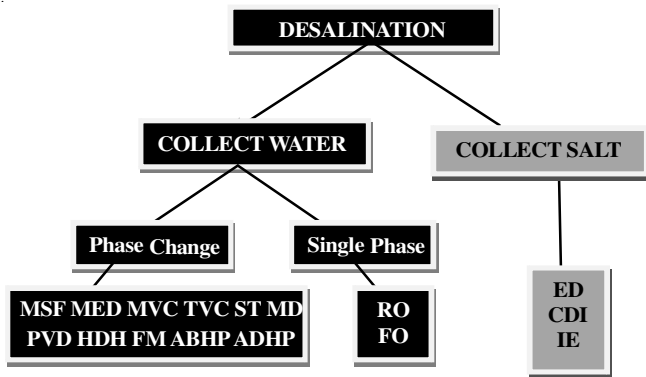
Fig. 3. Classification of desalination process [Ref. 10]
