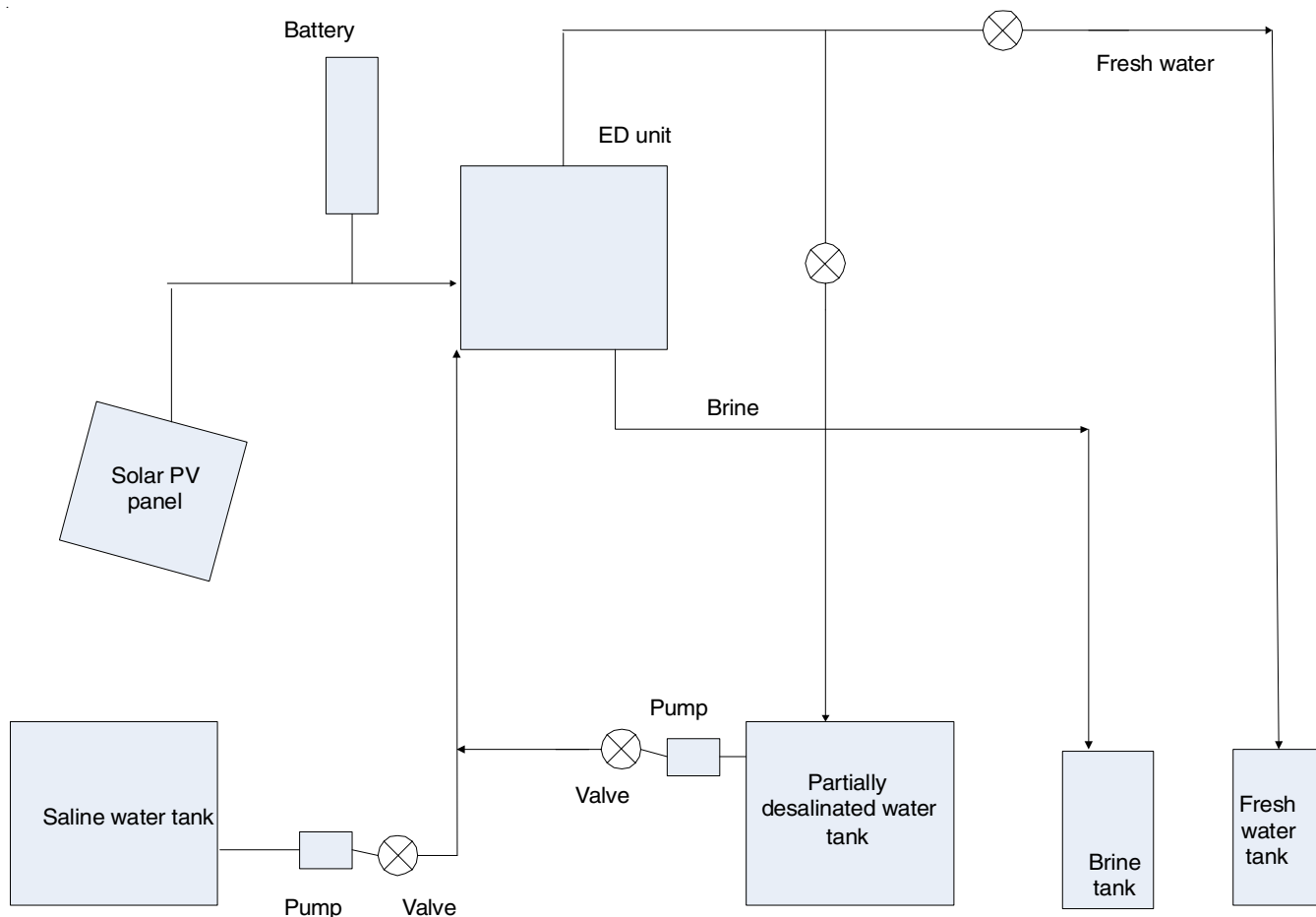
Fig. 8. Solar PV powered ED unit [Ref. 7]
