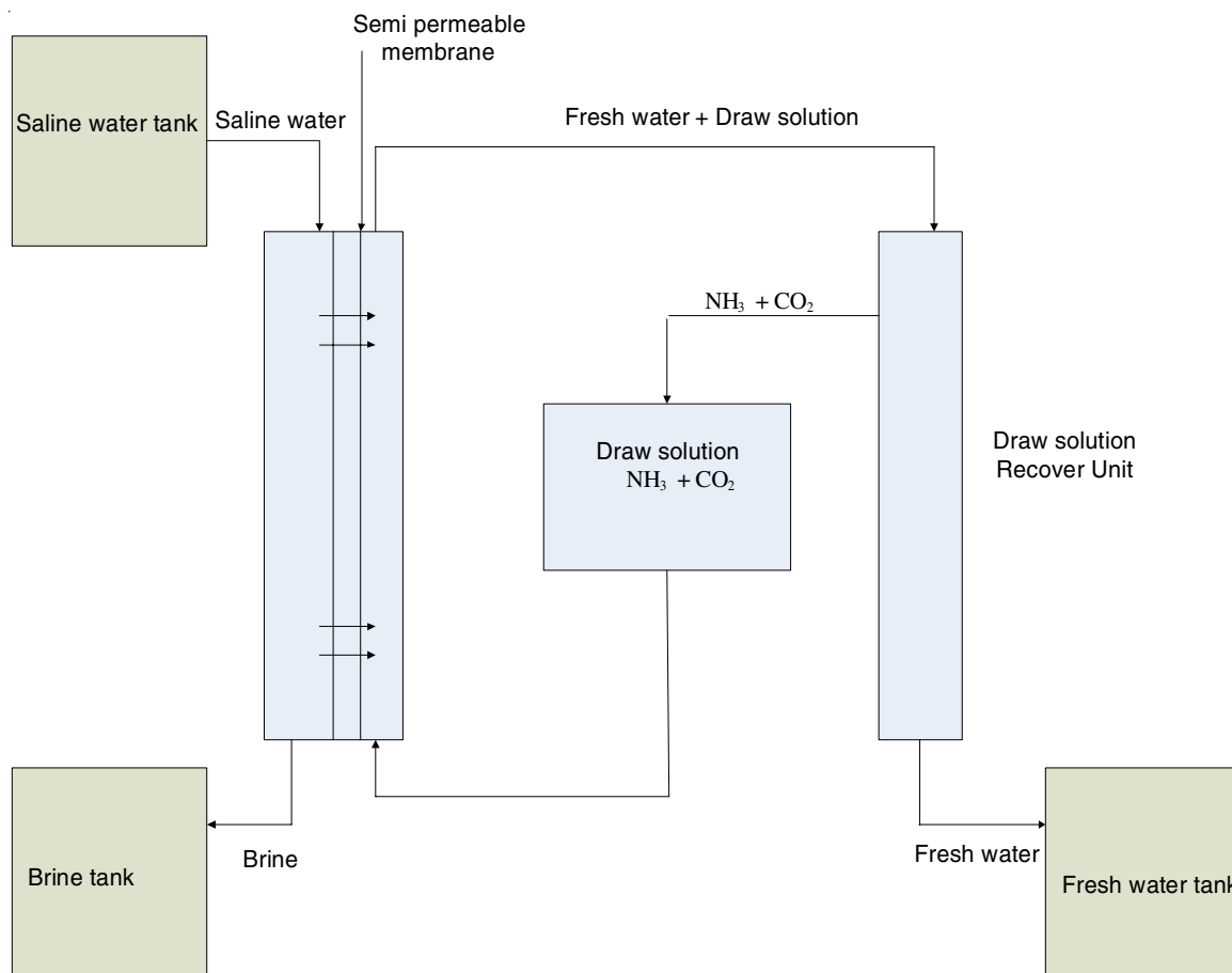
Fig. 11. Forward osmosis unit using \text{NH}_3\text{-CO}_2 as draw solution [Ref. 7]
