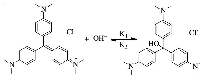
Scheme-I: Hydrolysis of crystal violet in the presence of [\text{OH}^-]
