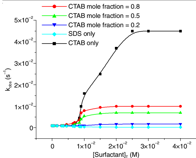
Fig. 1. Relationship of the observed rate constant, k_{obs} with the surfactant concentration for the alkaline hydrolysis of 1.5 \times 10^{-5} \text{ mol dm}^{-3} \text{CV}^+ on total surfactant concentration, [\text{Surfactant}]_T at 298 K for CTAB + SDS
