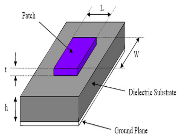
FIG. 1. SIMPLEST STRUCTURE
