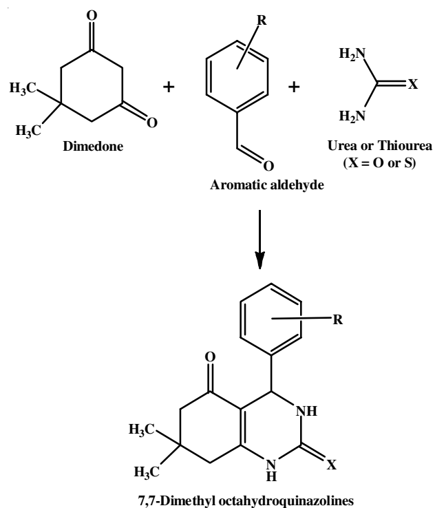
Scheme-I: Synthesis of various substituted dimethyl octahydroquinazolines using copper oxide nanoparticles
