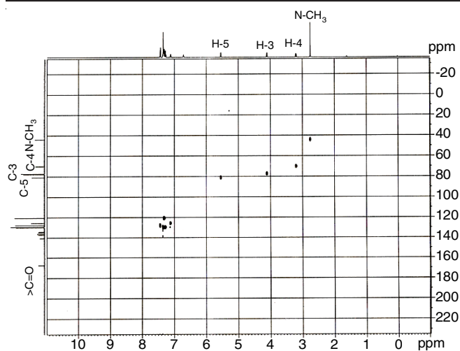
Fig. 5. 500 MHz ^1\text{H} NMR/125.5 MHz ^{13}\text{C} NMR heteronuclear shift correlation spectrum of compound 5a in \text{CDCl}_3 using the HMQC sequence
