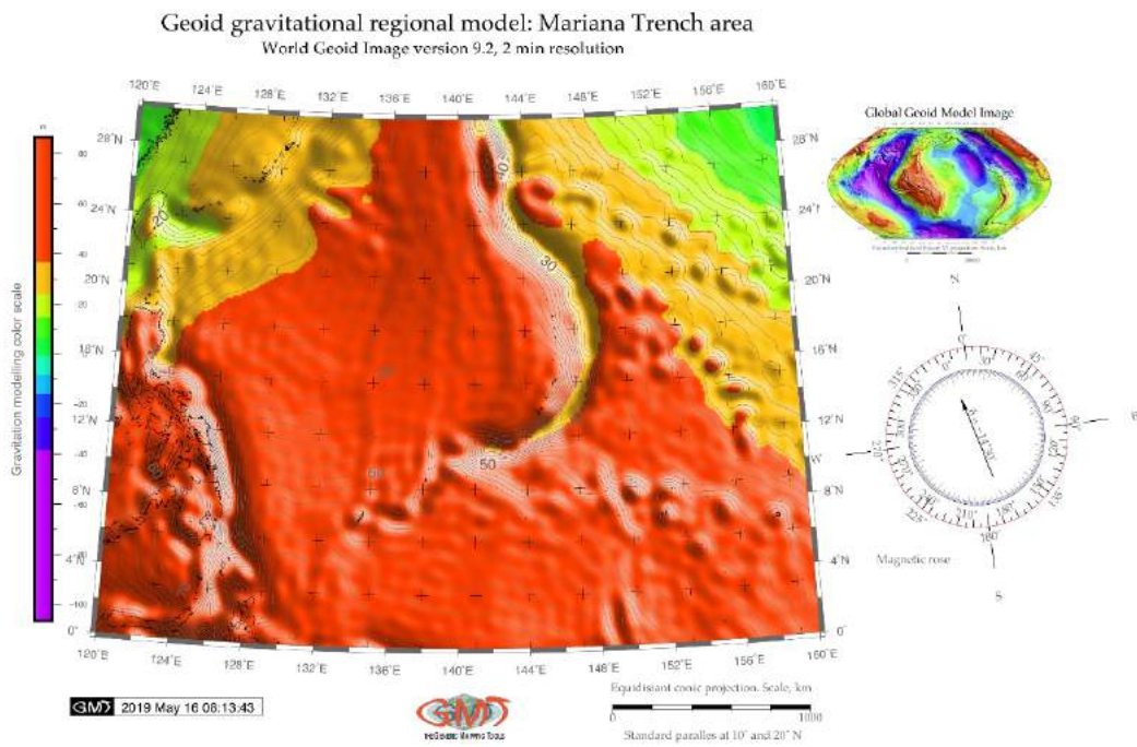
Fig. 3. Geoid modelling of the study area
