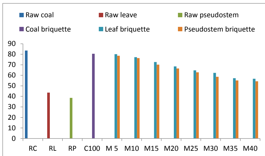
Fig. 5 - Carbon content of raw materials and produced briquettes
