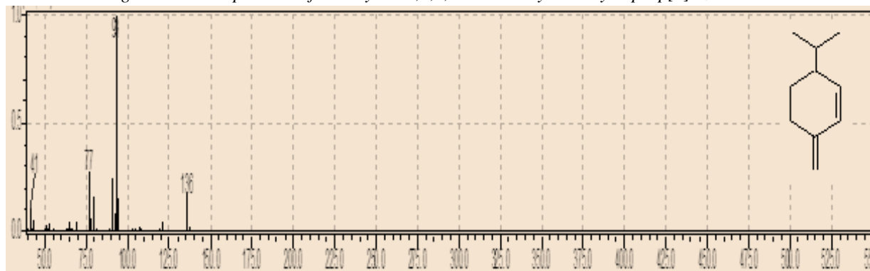
Figure 6: Mass spectrum of \beta -phellandrene
