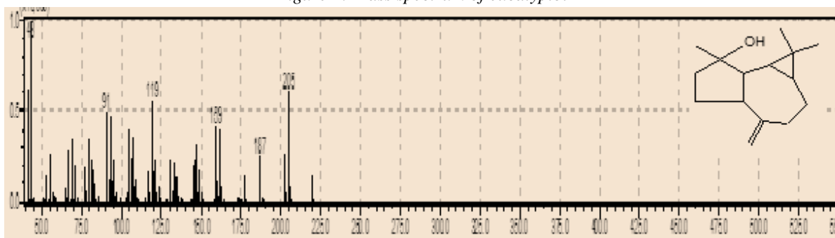
Figure 3: Mass Spectrum of decahydro-1,1,7-trimethyl-4-methylene - 1H-cycloprop[e]azulen-7-ol
