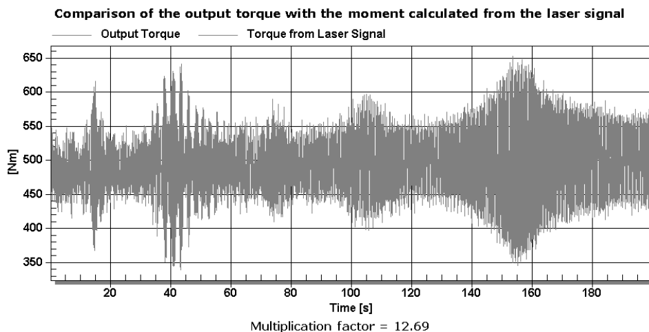
Fig. 6. Comparison of both torques as a function of time for the factor k=12.69
