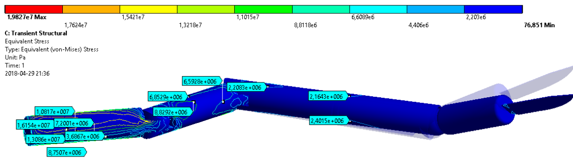
Fig. 5. The value of the reduced stress according to the Huber hypothesis for transient states in the iso-stress chart for movement in the first joint
