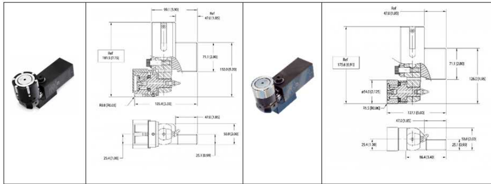
a. Multi Roller Burnishing Tool
