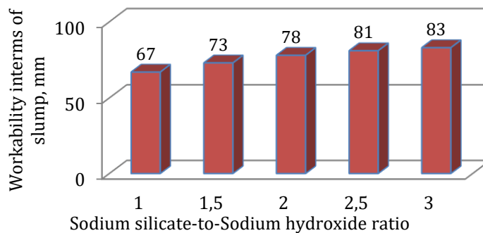
Fig. 2. Effect of alkaline ratio on workability (slump value) of geopolymer concrete
