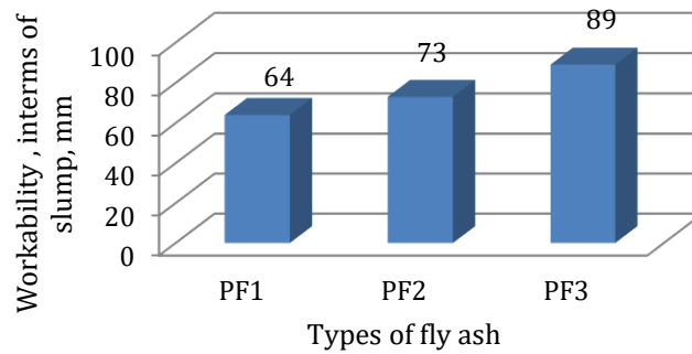
Fig.1. Effect of finesse of flyash on workability (slump value) of geopolymer concrete.
