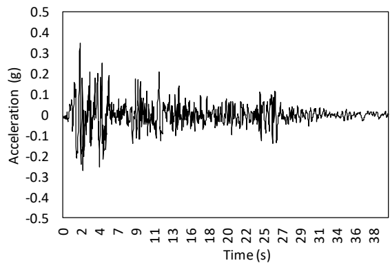
Fig. 3 El Centro accelerogram scaled for ground acceleration PGA = 0.349g
