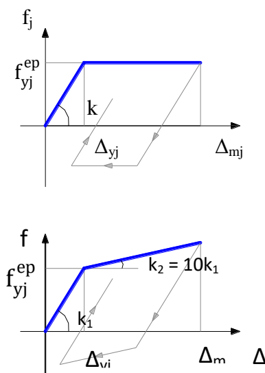
Fig. 9 Nonlinear diagram of elements:
