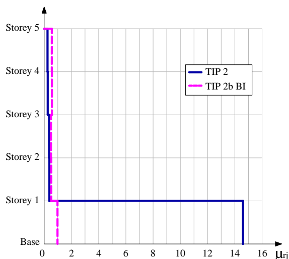
Fig. 10b The required ductility for each storey of fixed base (TYPE 2) and base isolated (TYPE 2b BI) of existing buildings) designed with allowable ductility \mu_a = 4
