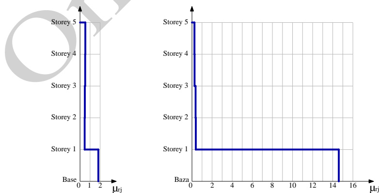
Fig. 7 . Required story ductility of TYPE 2 structure: a) for \mu_a=1 , b) for \mu_a=4
