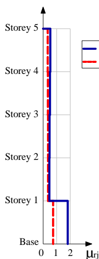
Fig. 10a The required ductility for each storey of fixed base (TYPE 2) and base isolated (TYPE 2a BI) of new structures designed with allowable ductility \mu_a = 1 .
