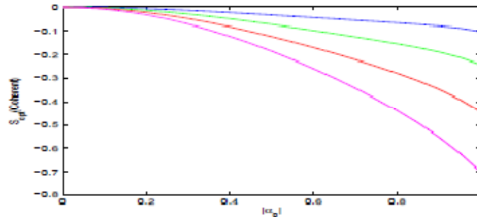
Fig. 7 Plot for S_{opt} as a function of |\alpha_0| with coherent state input and \lambda_n \sim [n]!
