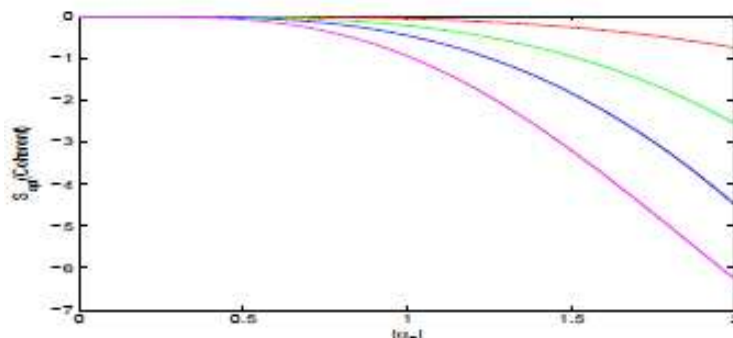
Fig. 5 Plot for S_{opt} as a function of |\alpha_0| with coherent state input and \lambda_n \sim n!
