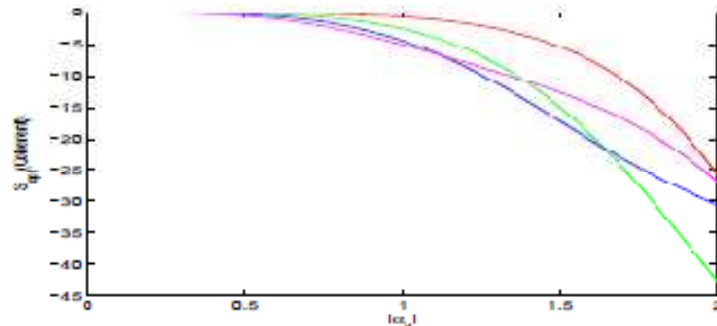
Fig. 6 Plot for S_{opt} as a function of |\alpha_0| with coherent state input and \lambda_n \sim (n!)^2
