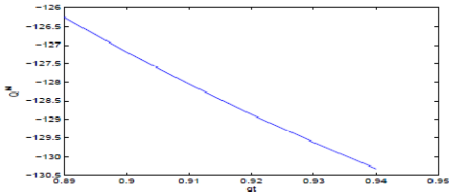
Fig. 4 Mandel's QM as a function of gt for a coherent state input and \lambda_n \sim n!
