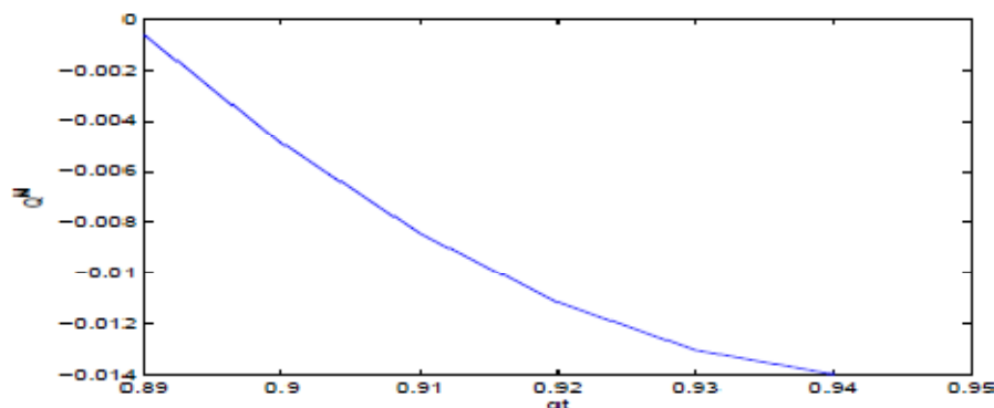
Fig. 2 Mandel's QM as a function of gt for a coherent state input and \lambda_n \sim n!
