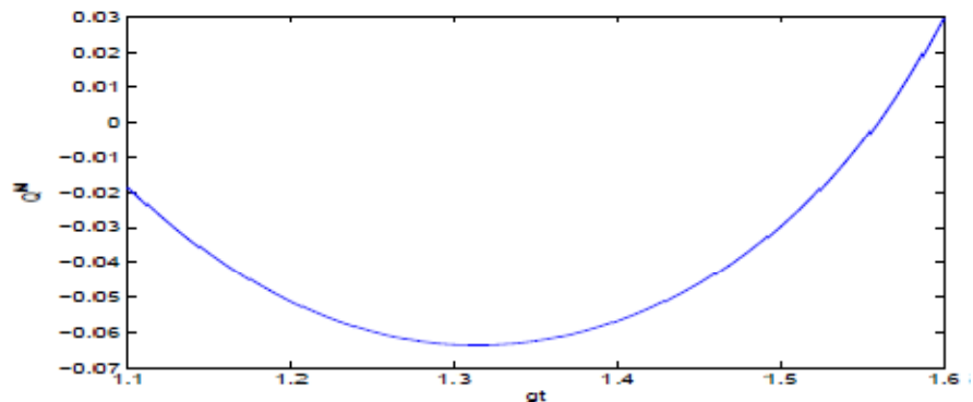
Fig. 3 Mandel's QM as a function of gt for a coherent state input and \lambda_n \sim n!^2
