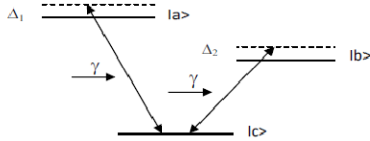
Fig. 1 Energy diagram of a vee-configuration three-level atom interacting with one quantized cavity mode
