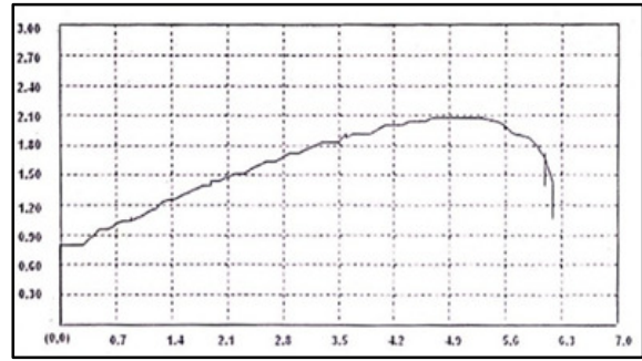
Fig.17. Load Vs Displacement graph for Specimen FR-II
