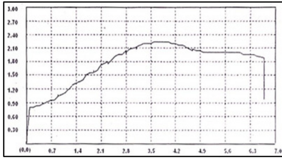
Fig.13. Load Vs Displacement graph for Specimen AL-III
