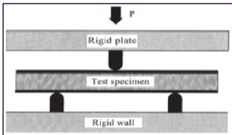
Fig.1. Bending Test Set-up [5]
