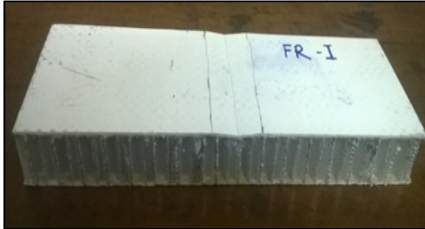
Fig.14. Specimen FR-I of GFRP – Polypropylene panel after bending
