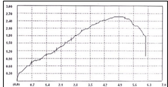
Fig.11. Load Vs Displacement graph for Specimen AL-II
