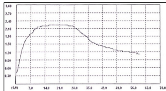
Fig.3. Load Vs Displacement graph for Specimen SS-I
