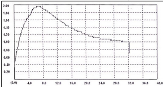
Fig.7. Load Vs Displacement graph for Specimen SS-III
