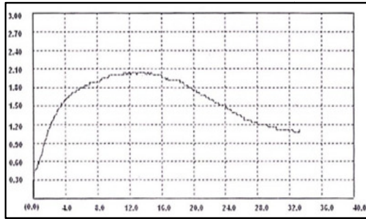
Fig. 5 Load Vs Displacement graph for Specimen SS-II
