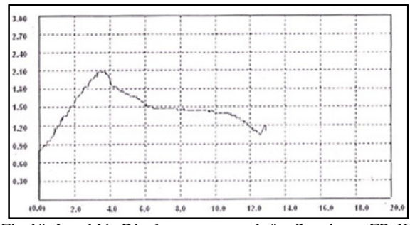
Fig.19. Load Vs Displacement graph for Specimen FR-III
