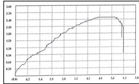
Fig.9. Load Vs Displacement graph for Specimen AL-I
