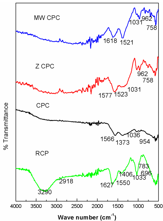
Figure 4. FT-IR Spectra of RCP, CPC, Z CPC and MW-CPC.
