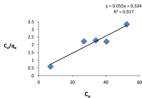
Figure 7. Linear transform of Langmuir isotherm [BaBiO 3 =0.75gL -1 ; pH=6.0]
