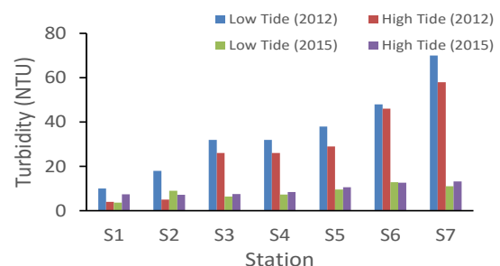
Figure 7. Turbidity at seven sampling stations for low tide and high tide of 2012 and 2015
