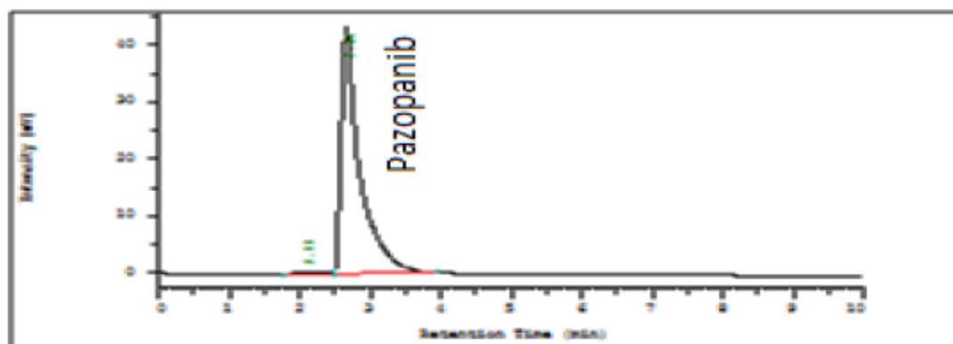
Figure 2: Standard Chromatogram.
