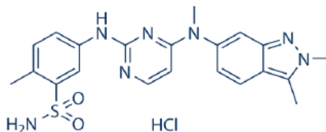
Figure 1: Chemical structure of Pazopanib hydrochloride.
