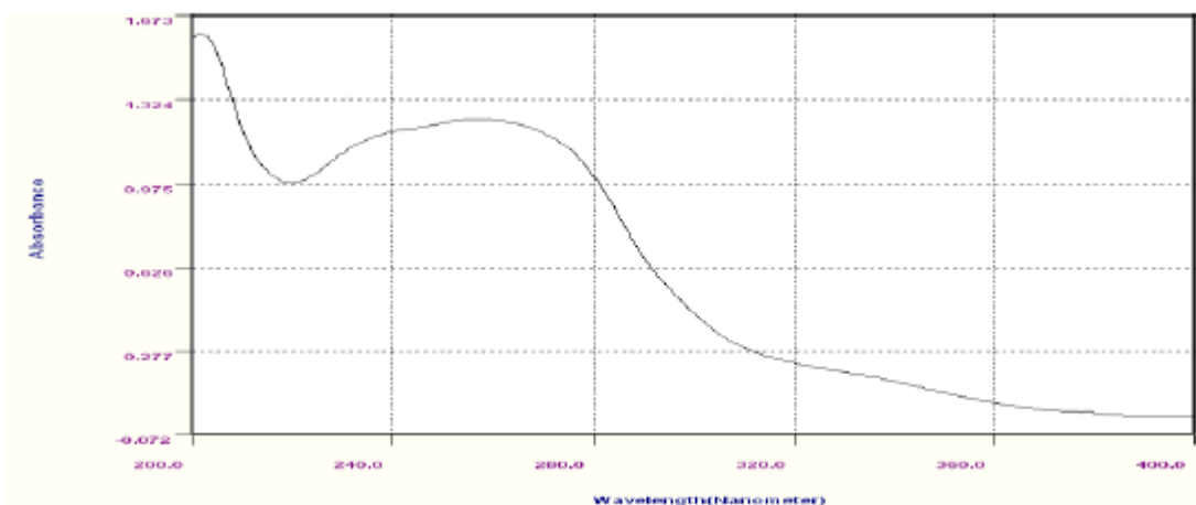
Figure 4: UV spectrum of Pazopanib hydrochloride.
