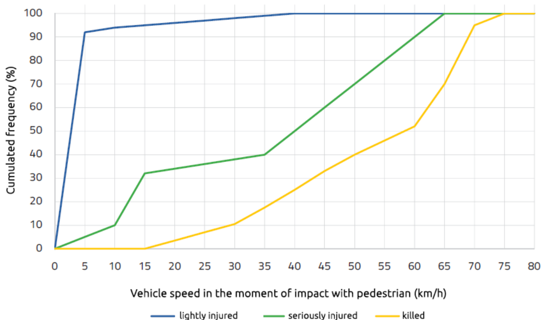
Fig. 1. Results of vehicle-pedestrian collision at various speeds: cumulative amounts (in percentages) of lightly wounded (blue), severely wounded (green) and killed (yellow) are shown [Błąd! Nie zdefiniowano zakłádki.]
