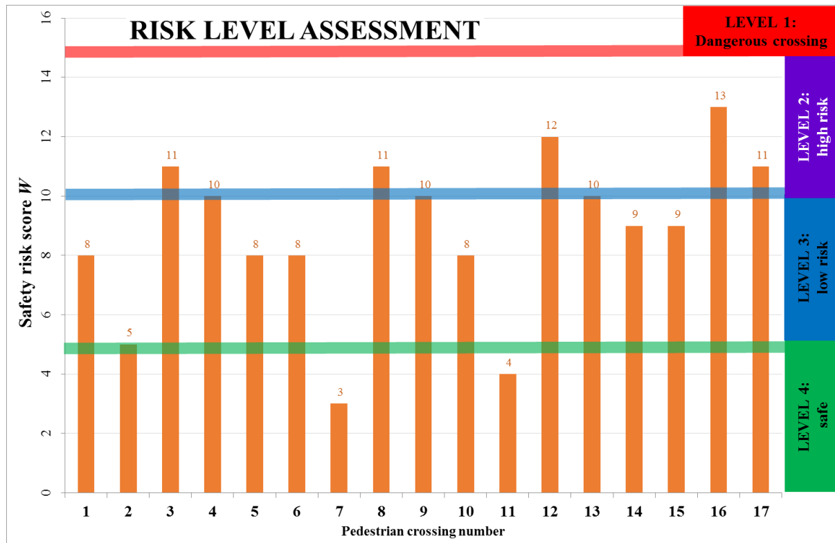
Fig. 3. Safety risk assessment of pedestrian crossings in Sulkowice; safety risk score W
