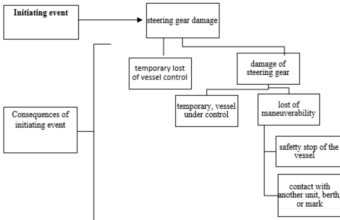
Fig. 3. Hazard identification model constructed using ETA techniques
