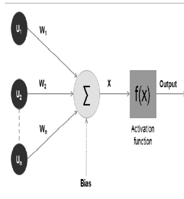
Fig (1): Mathematical model of artificial neuron
