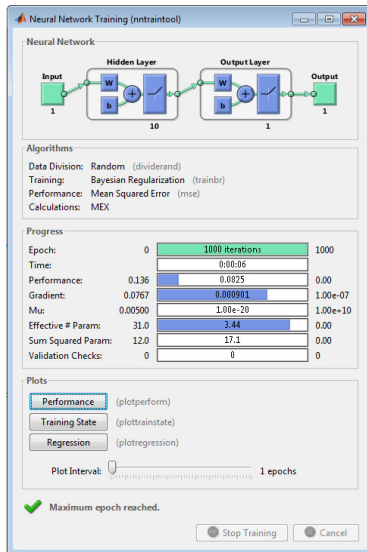
Fig(16) Training with Poslin transfer function for hidden and output layers
