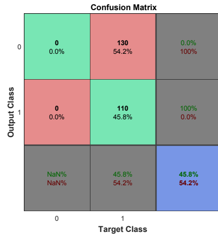
Fig (6) Confusion matrix for GDM learning algorithm
