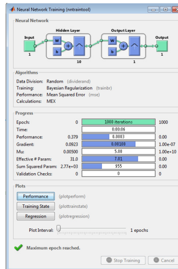
Fig(15) Training with Radbas function for hidden and output layers
