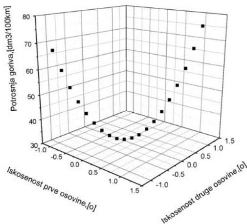
Slika 9 – Uticaj uglova iskošenosti osovina na potrošnju goriva pri brzini od 57,10 km/h i usponu od 0,15% (peti stepen prenosa) Figure 9 – Influence of axle inclination angles on fuel consumption at a speed of 57.10 km/h, and on a gradient of 0.15% (fifth gear)
