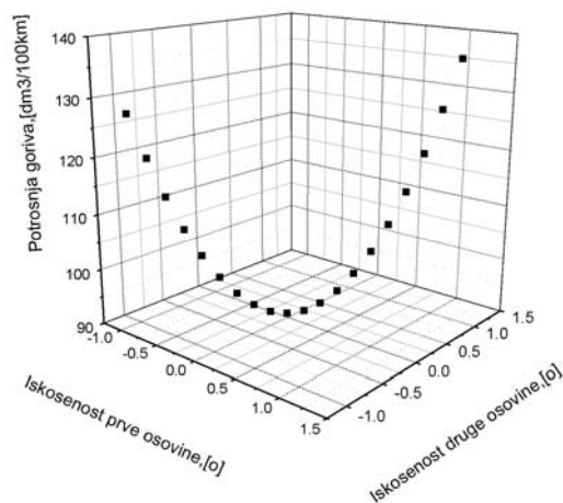
Slika 8 – Uticaj uglova iskošenosti osovina na potrošnju goriva pri brzini od 21,79 km/h i usponu od 2,45% (treći stepen prenosa) Figure 8 – Influence of axle inclination angles on fuel consumption at a speed of 21.79 km/h, and on a gradient of 2.45% (third gear)
