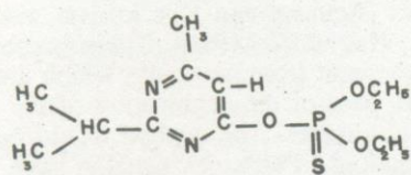
Diazinon
