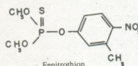
Fenitrothion
