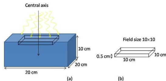
Fig.5. Schematic diagram of a) water phantom and b) a cell defined inside water to calculate absorbed dose rate in a depth of 0.5 cm by MCNP code.
