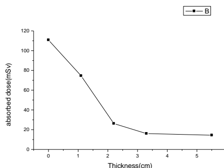
Fig.6. Absorbed dose rate variations in heart region versus lead powder thickness. As seen, about 3cm thickness is suitable to reduce dose rate in heart.
