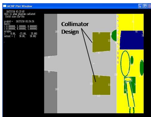
(b) Fig.8. plot of designed collimator that extracted from output file of MCNP code
