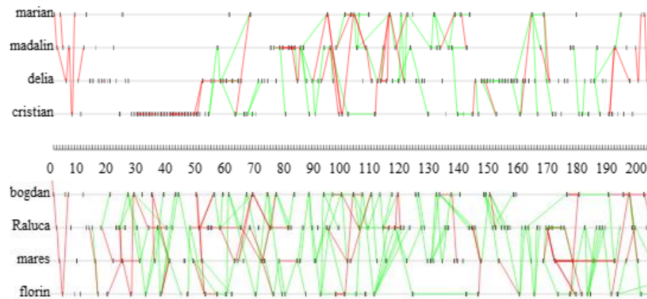
Figure 3. Comparative view of the network of explicit (red) and implicit (green) arcs among utterances. Obviously in the bottom case inter-animation is probably considerably higher. The visualization (type B135) was done with the PolyCAFe system
