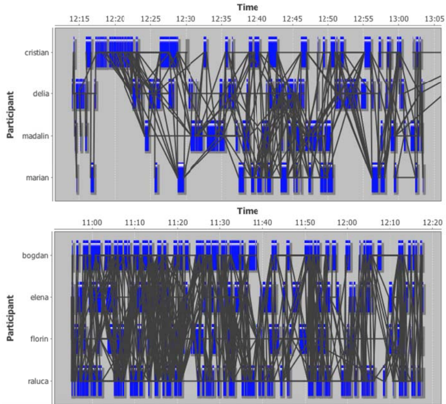
Figure 4. Comparative view of the conversation graphs in ReaderBench . In addition to the PolyCAFe system, more implicit links are detected considering cohesion among utterances
