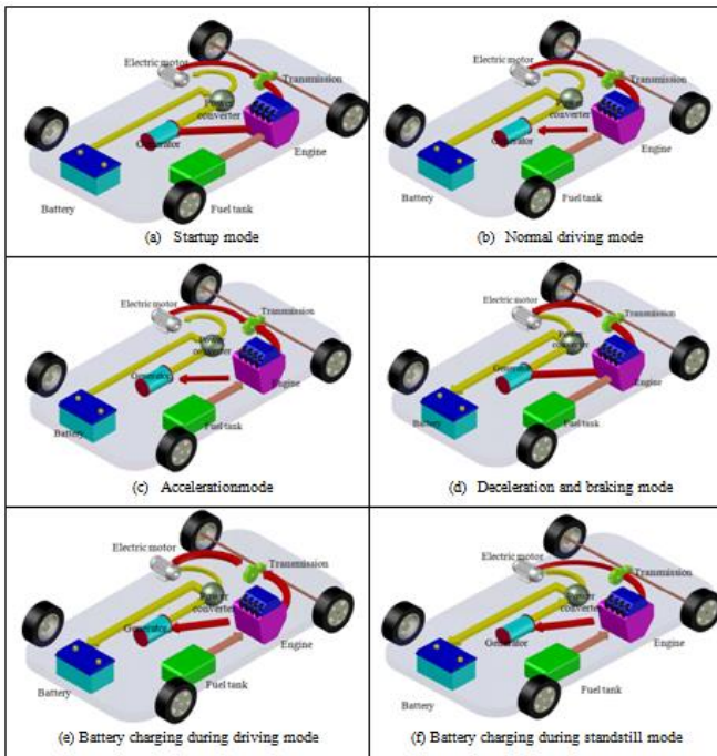
Figure 4: Series - parallel hybrid electric vehicle operating modes (Electric – Heavy operating mode).
