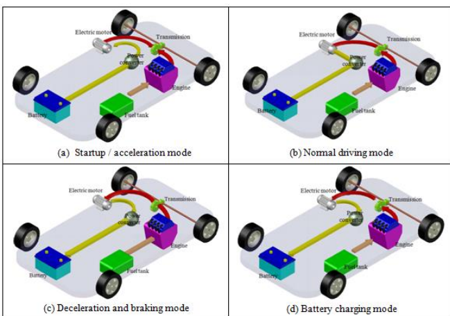
Figure 2: Parallel hybrid electric vehicle operating modes.
