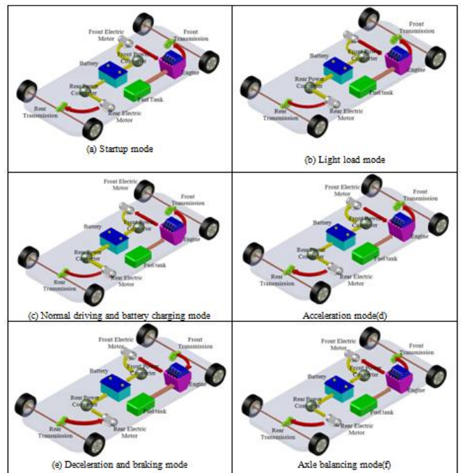
Figure 5: Dual axle complex hybrid electric vehicle operating modes (front - hybrid drive train, and the rear - electric motor).
