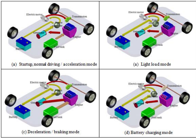
Figure 1: Series hybrid electric vehicle operating modes.
