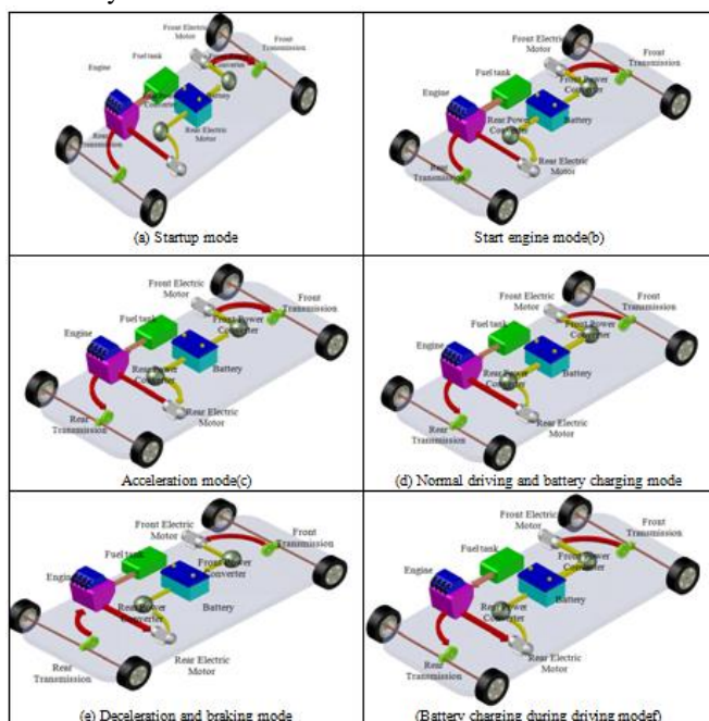
Figure 6: Dual axle complex hybrid electric vehicle operating modes (front - electric motor, and the rear hybrid drive train).
