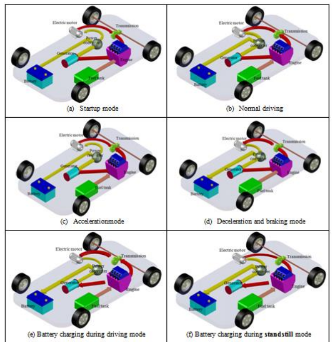
Figure 3: Series - parallel hybrid electric vehicle operating modes (Engine – Heavy operating mode).
