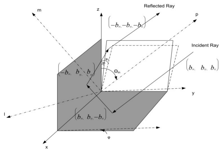
Figure 4. Structure of TCCR
