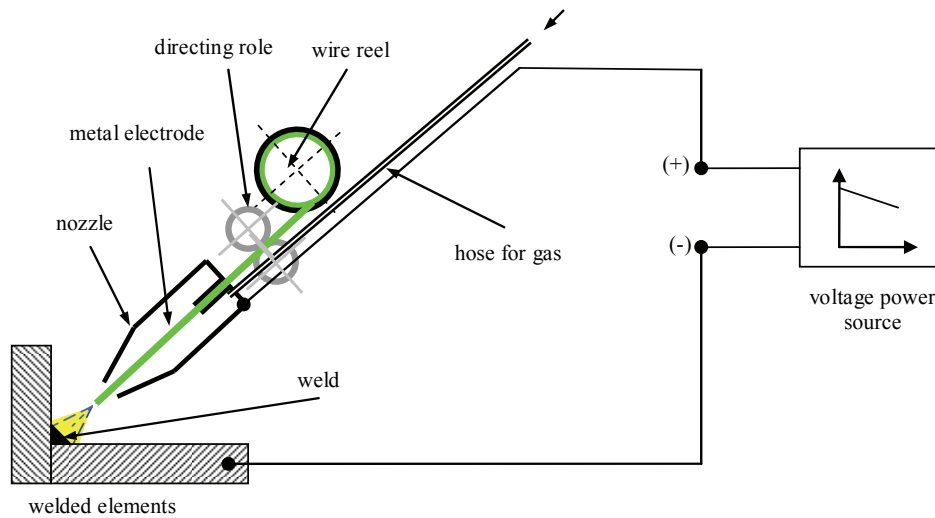
Fig. 3 - Draft of metal inert gas (MIG) and metal active gas (MAG) welding (Pilarczyk 2003)
