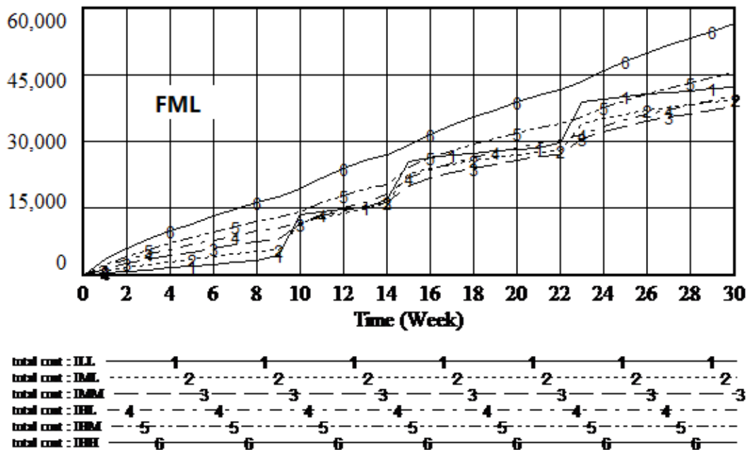
Figure 11: Total cost of different inventory policies with transshipment when disaster frequency is medium & low
