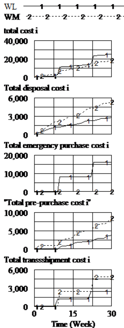
Figure 18: Cost comparing for different inventory policy with transshipment
