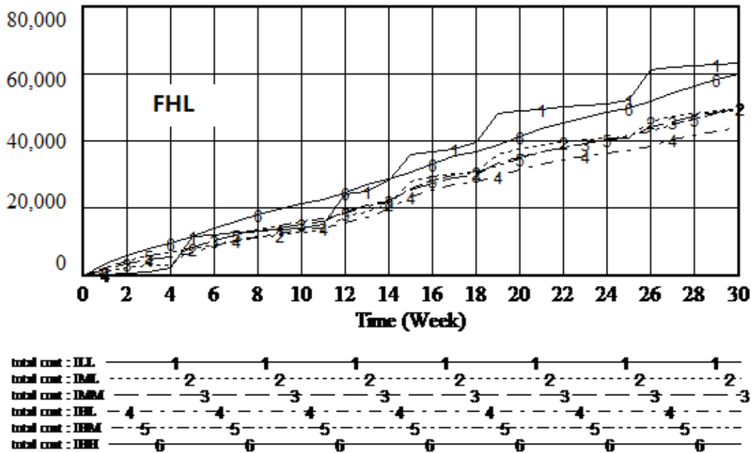
Figure 14: Total cost of different inventory policies with transshipment when disaster frequency is high & low
