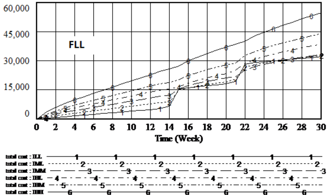
Figure 8: Total cost of different inventory policies with transshipment when disaster frequency is low & low
