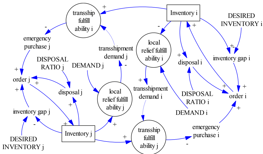
Figure 4: Causal loop diagram of transshipment
