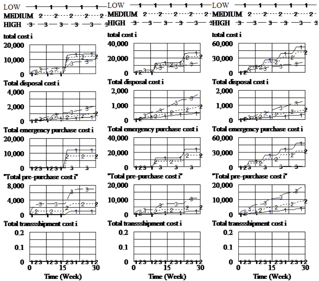
Figure 7: Cost of different inventory policy without transshipment
