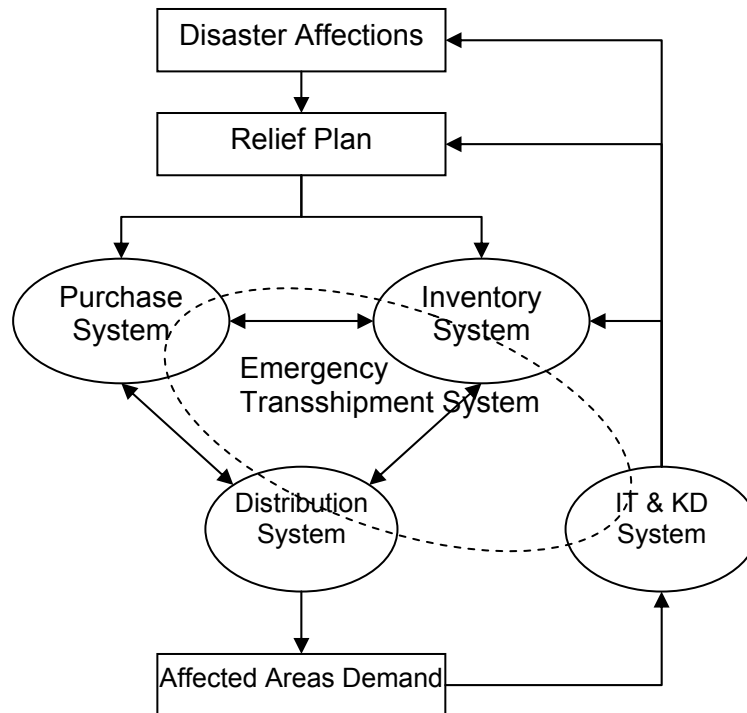
Fig.2. Framework of Relief Supply Decision System
