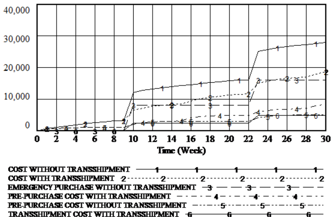
Figure 19: Cost structure with and without transshipment
