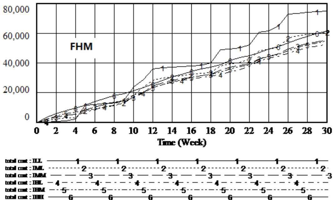
Figure 15: Total cost of different inventory policies with transshipment when disaster frequency is high & medium
