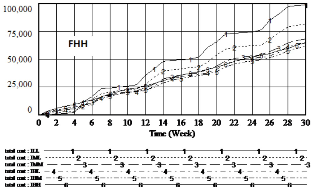
Figure 16: Total cost of different inventory policies with transshipment when disaster frequency is high & high
