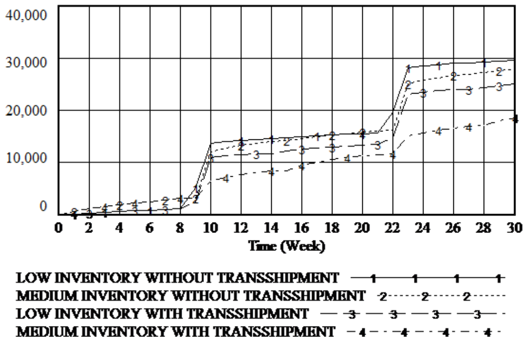
Figure 17: Total cost with and without transshipment
