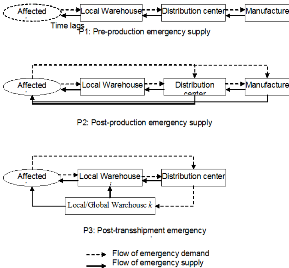
Fig 1. Three Basic Emergency supply patterns
