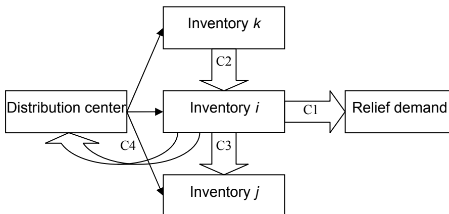
Fig 3. Inventory structure of single warehouse based on transshipment
