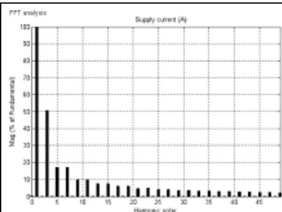
FIG. 12. SIMULATED SUPPLY CURRENT HARMONIC FOR A 90° FIRING ANGLE BIDIRECTIONAL AC VOLTAGE CONTROLLER
