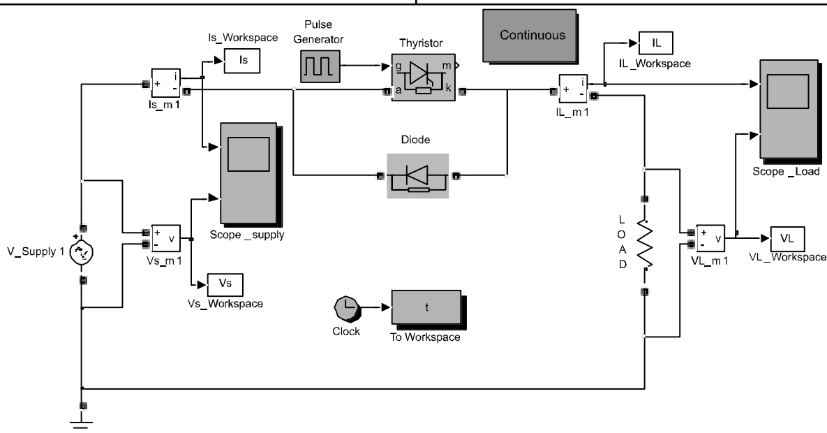
FIG. 3. SIMULATION MODEL OF UNIDIRECTIONAL AC VOLTAGE CONTROLLER.
