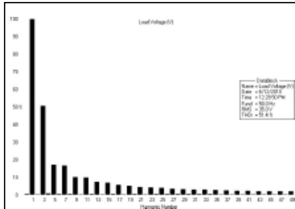
FIG. 17. EXPERIMENTAL LOAD VOLTAGE HARMONIC FOR A 90° FIRING ANGLE OF BIDIRECTIONAL AC VOLTAGE CONTROLLER
