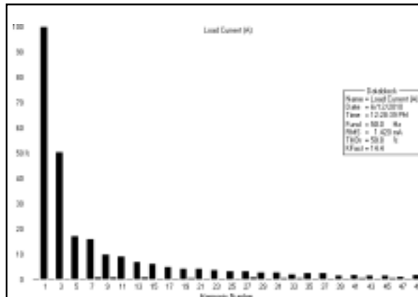
FIG. 15. EXPERIMENTAL LOAD CURRENT HARMONIC FOR A 90° FIRING ANGLE OF BIDIRECTIONAL AC VOLTAGE CONTROLLER
