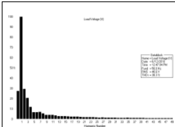
FIG. 7. SIMULATED LOAD VOLTAGE HARMONIC FOR A 90° FIRING ANGLE UNIDIRECTIONAL AC VOLTAGE CONTROLLER
