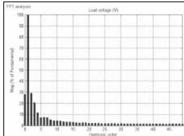
FIG. 8. EXPERIMENTAL LOAD VOLTAGE HARMONIC FOR A 90° FIRING ANGLE OF UNIDIRECTIONAL AC VOLTAGE CONTROLLER
