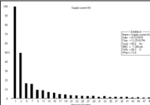
FIG. 13. EXPERIMENTAL SUPPLY CURRENT HARMONIC FOR A 90° FIRING ANGLE OF BIDIRECTIONAL AC VOLTAGE CONTROLLER
