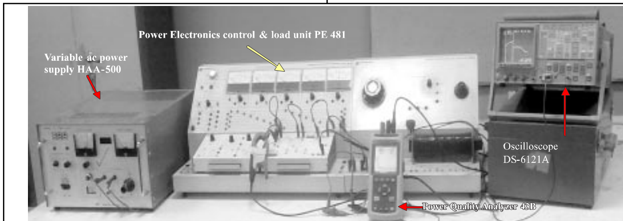
FIG. 9. EXPERIMENTAL SETUP OF AC VOLTAGE CONTROLLERS
