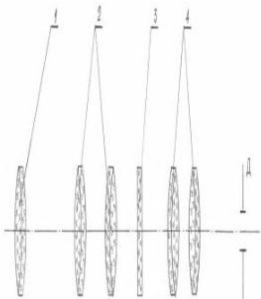
Fig. 2. Optical system of "Vizir – target 15 K"
