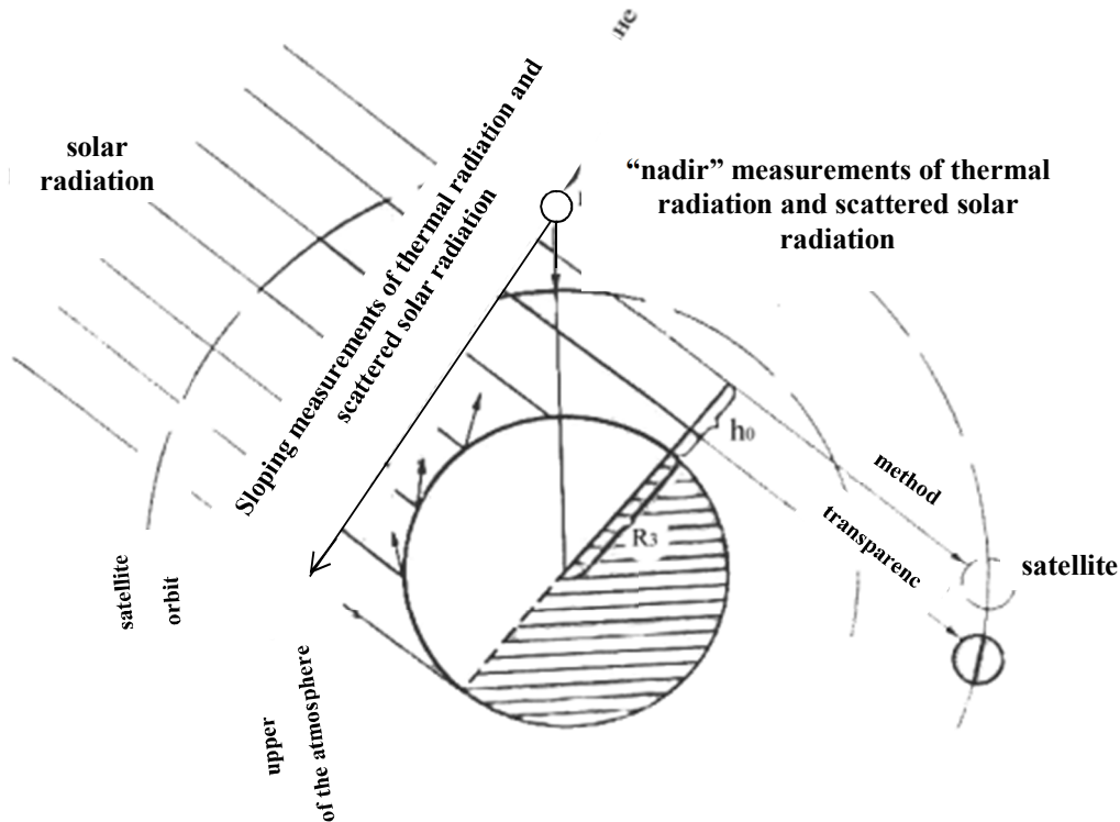
Fig. 1. Satellite passive methods and geometry of measurements of TGC ( h_0 - informative height, R_3 - the radius of the Earth)
