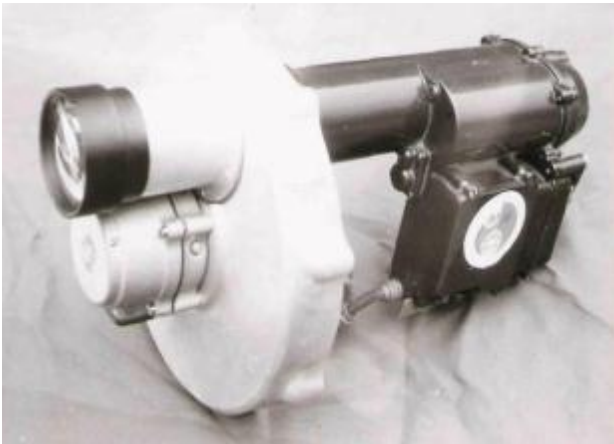
Fig. 7. Electron optical viewfinder for testing of particular atmospheric emissions in the near infrared part of the optical spectrum
