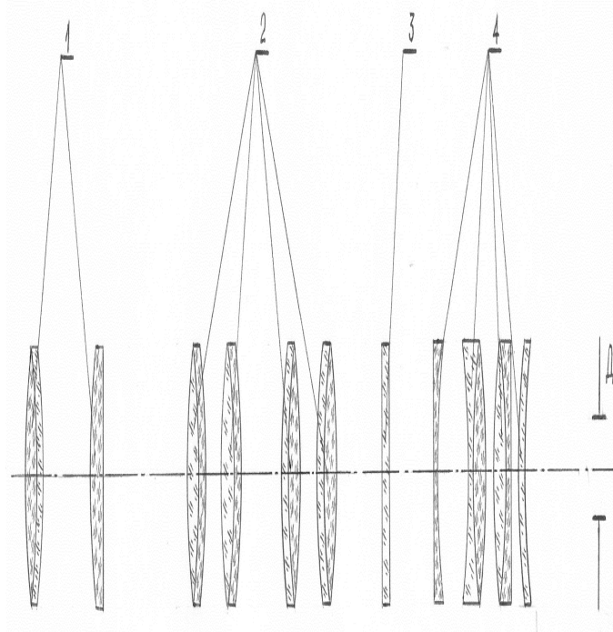
Fig. 4. Optical system of Vizir B3x40
