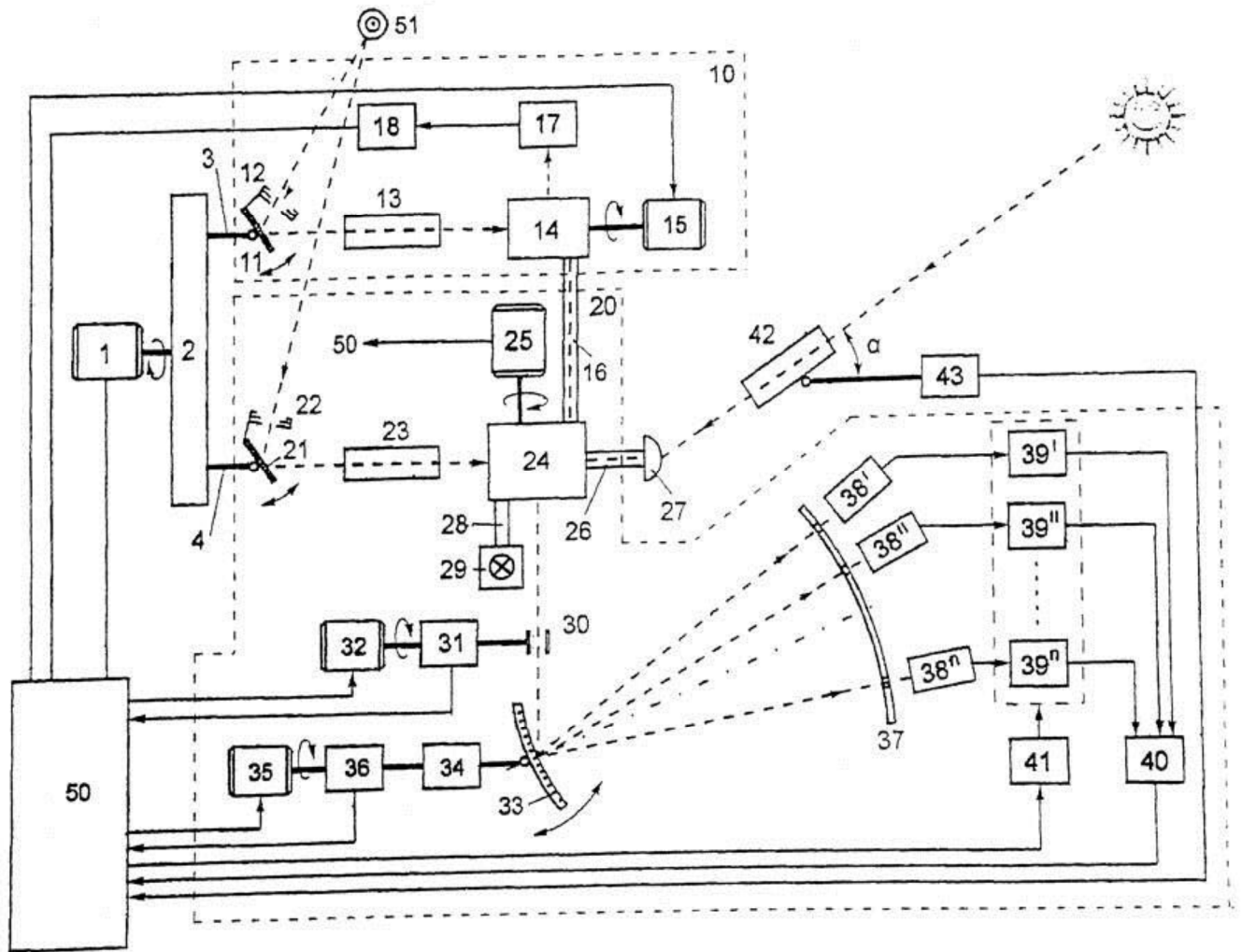
Fig. 11. A spectrophotometer for monitoring of the atmosphere
