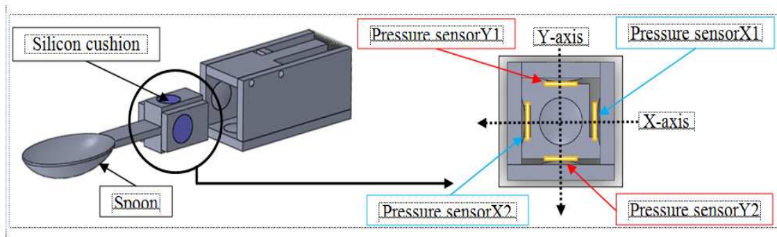
Figure 2: Disposition of Four Pressure Sensors
