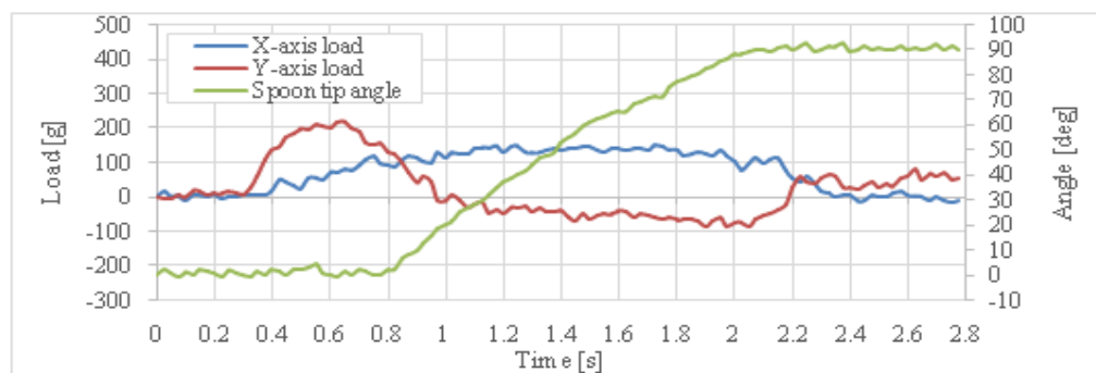
Figure 5: Transition of Load Values of X-Axis and Y-Axis, and Spoon Tip Angle; Trial Subject of Food, Fried Rice; Rotational Speed, 0.25[rps]
