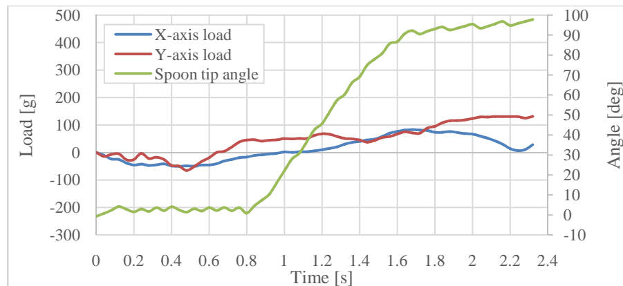
Figure 12: Transition of Load Values of X-Axis and Y-Axis, and Spoon Tip Angle; Trial Subject of Food, Jelly; Rotational Speed, 0.375[RPS]
