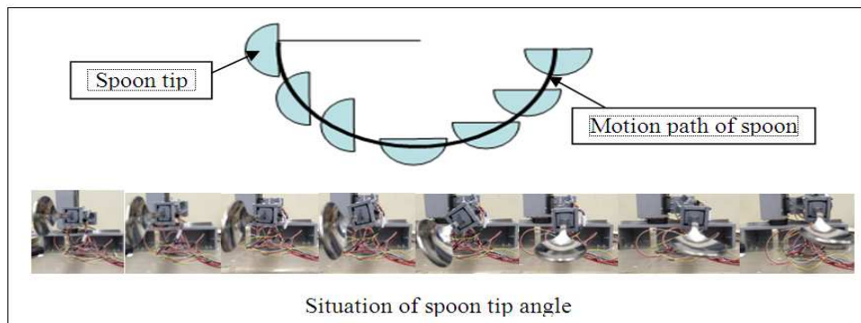
Figure 3: The Transition of the Spoon tip of Spoon When the Measuring Equipment Spoons up Foods
