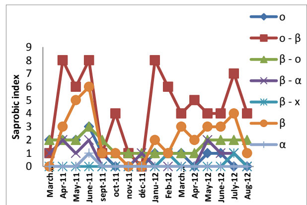
Figure 2: Temporal variation of the saprobic index during investigation period.
