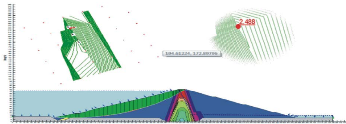
Fig. 5: Simulated model of Alavian dam and stability safety factor (present dam)
