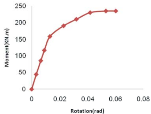
Fig. 3: Moment- rotation curve for component method
