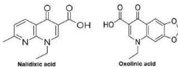
Fig. 4: Chemical structure of template and template analog molecules
