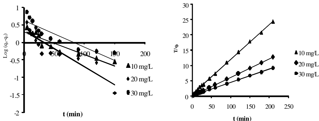
Fig. 6: (a) Pseudo-first-order (b) Pseudo-second-order kinetic plots for biosorption of CV onto CLR at different initial concentrations (particle size=150-300 \mu m; agitation speed=150 rpm; temperature =30°C)
