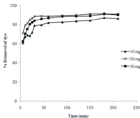
Fig. 5: Effect of contact time on biosorption of CV by CLR at different initial dye concentration (biosorbent dosage=1 g/L; particle size=150-300 \mu m; agitation speed=150 rpm; temperature=30°C)
