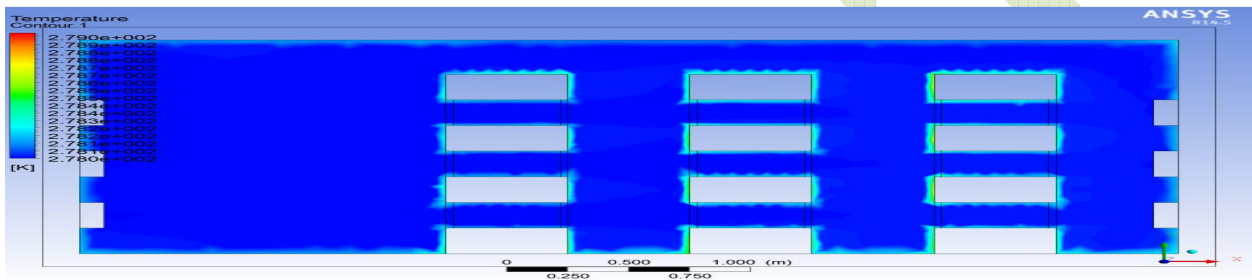
Fig.8.5.2 Temperature field of a cold store with 500 mm gap between racks
