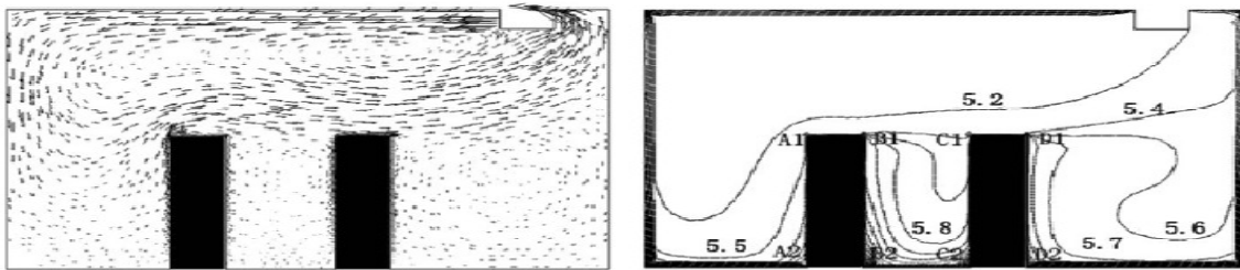
Fig.6.3 Previous work model of flow field and temperature field in the cold store for 6m/s
