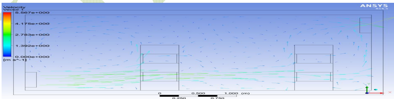
Fig.8.2.1 Flow field of a cold store with inlet at 100 mm and outlet at 1900 mm from base
