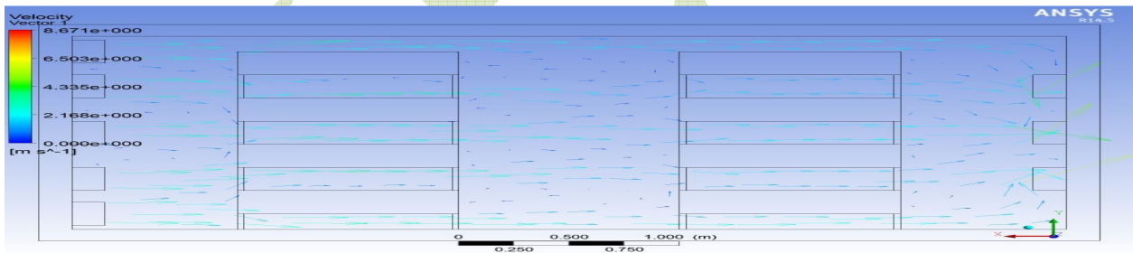
Fig.8.8.1 Flow field for design configuration 5 of a cold store
