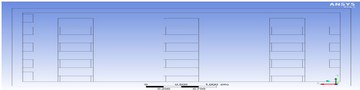
Fig.7.7 A cold store with 1000 mm gap between racks, an inlet at top and bottom of racks and air gap of 200 mm at bottom of racks
