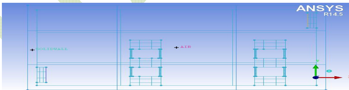
Fig.7.2 A cold store with inlet at 100 mm and outlet at 1900 mm from base
