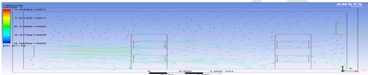
Fig.8.1.1 Flow field of a cold store with inlet at 500 mm and outlet at 1500 mm from base
