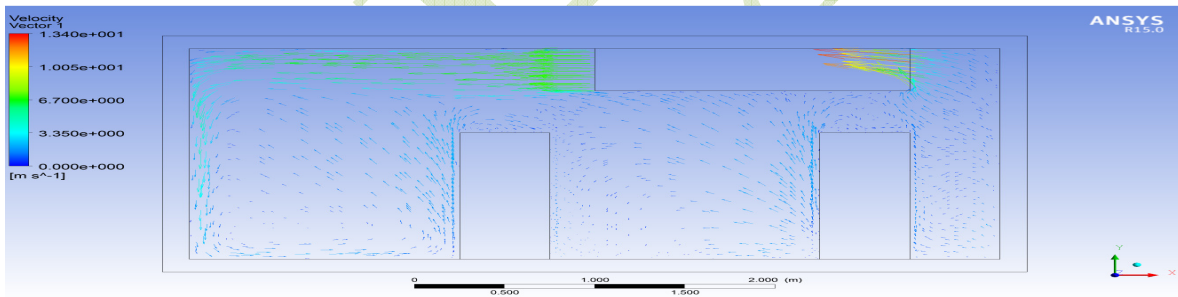
Fig.6.4 Present work model of flow field in the cold store for 6m/s
