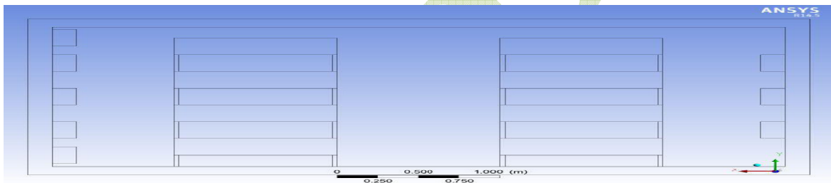
Fig.7.8 A cold store with 1000 mm gap between racks, inlets at top and bottom of racks and air gap of 200 mm at bottom of racks
