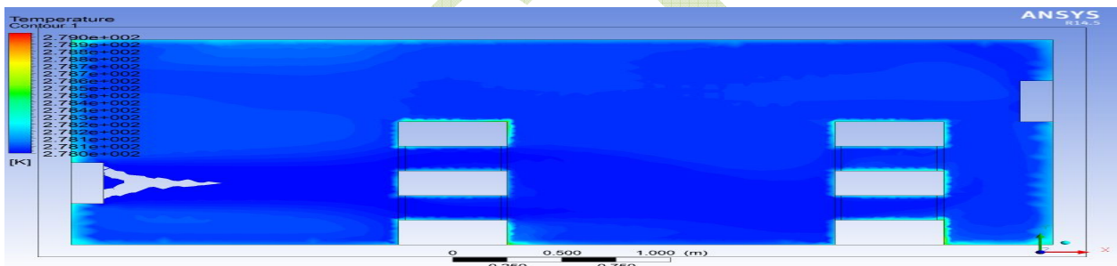
Fig.8.1.2 Temperature field of a cold store with inlet at 500 mm and outlet at 1500 mm from base
