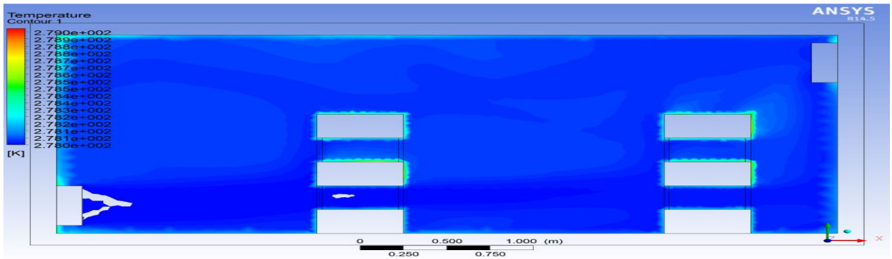
Fig.8.2.2 Temperature field of a cold store with inlet at 100 mm and outlet at 1900 mm from base
