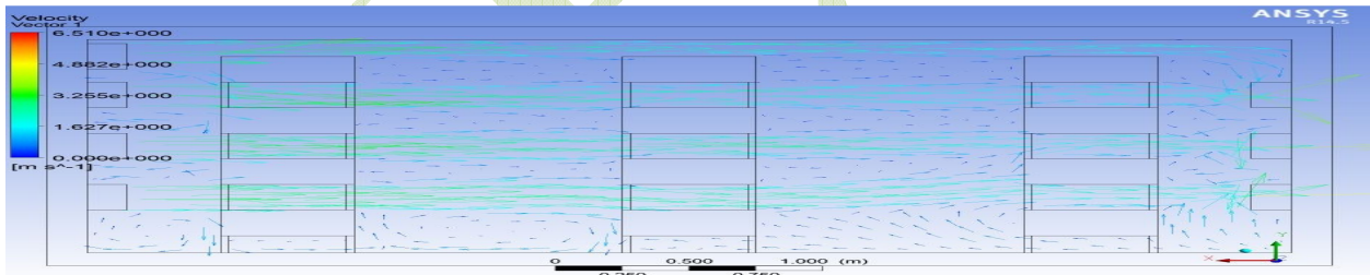
Fig.8.6.1 Flow field of a cold store with 1000 mm gap between racks, an inlet at top and air gap of 200 mm at bottom of racks
