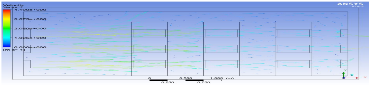
Fig.8.5.1 Flow field of a cold store with 500 mm gap between racks
