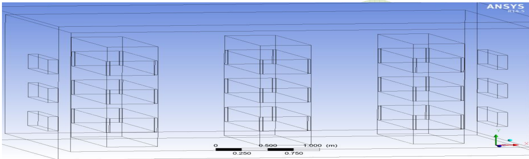
Fig.7.4A cold store with 1000 mm gap between racks
