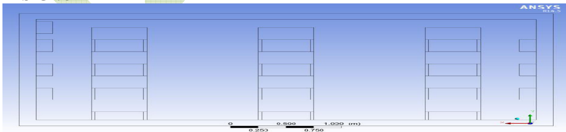
Fig.7.6 A cold store with 1000 mm gap between racks, an inlet at top and air gap of 200 mm at bottom of racks
