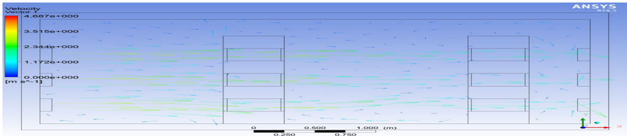
Fig.8.3.1 Flow field of a cold store with 1500 mm gap between racks
