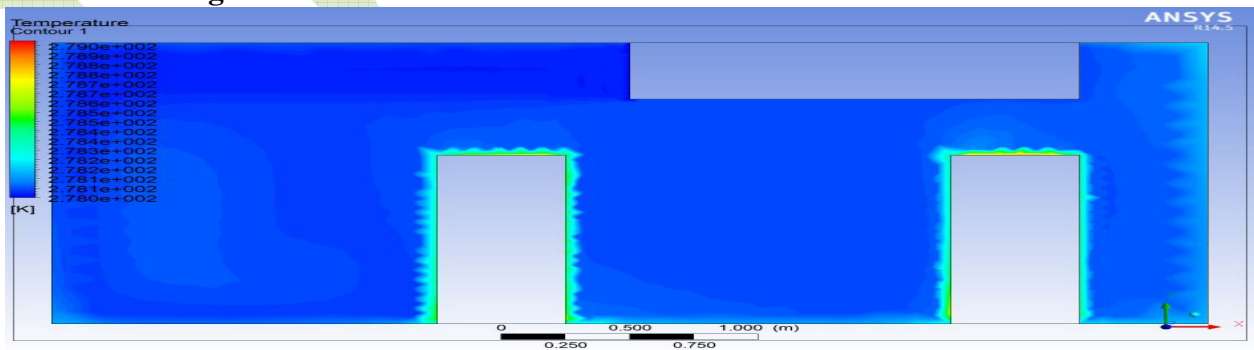
Fig.6.5 Present work model of temperature field in the cold store for 6m/s
