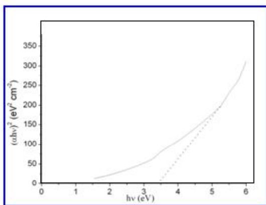
Fig. 4: Tauc plot for \text{TiO}_2
