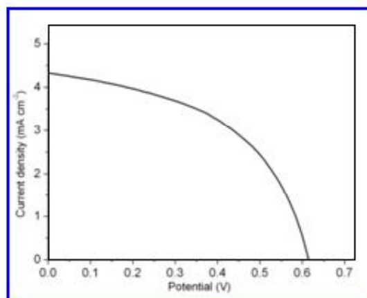
Fig. 5: I-V Characteristics of solar cell
