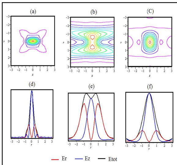
Fig. 2.(a & d) plane radially polarized beam, (b & e) radially polarized Lorentz gaussian beam for NA=0.95 , W=0.3 , \gamma=0.3 , (c & f) radially polarized Lorentz gaussian beam for W=0.3 , \gamma=1.2 , and m=0
