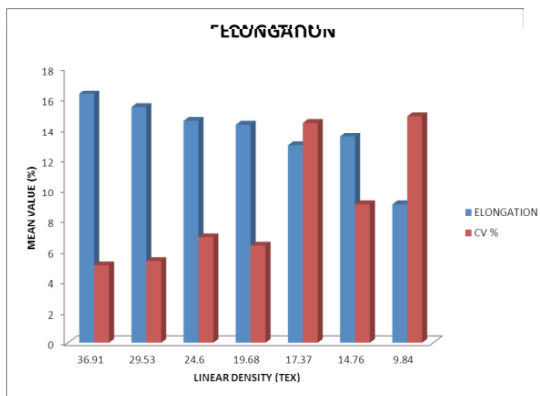
Fig. 6: Elongation & CV%
