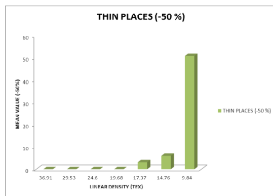
Fig. 9: Thin Places (-50%)
