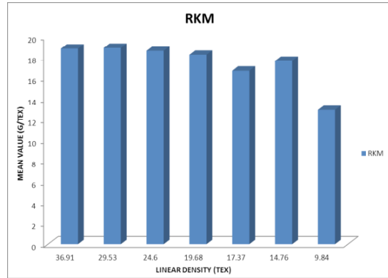
Fig. 7: RKM
