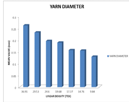
Fig. 13: Yarn Diameter
