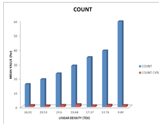
Fig. 2: Count & CV%
