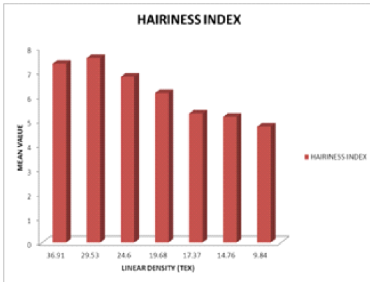
Fig. 12: Hairiness Index
