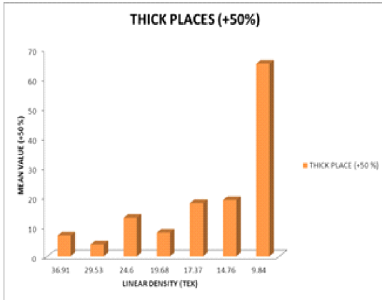
Fig. 10: Thick Places (+50%)
