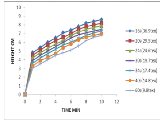
Fig. 14: Wicking Behaviour – Height & Time
