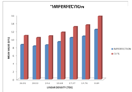
Fig. 8: Imperfection & CV%
