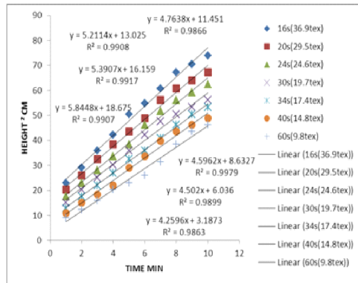
Fig. 15: Wicking Behaviour – Height Square and Time
