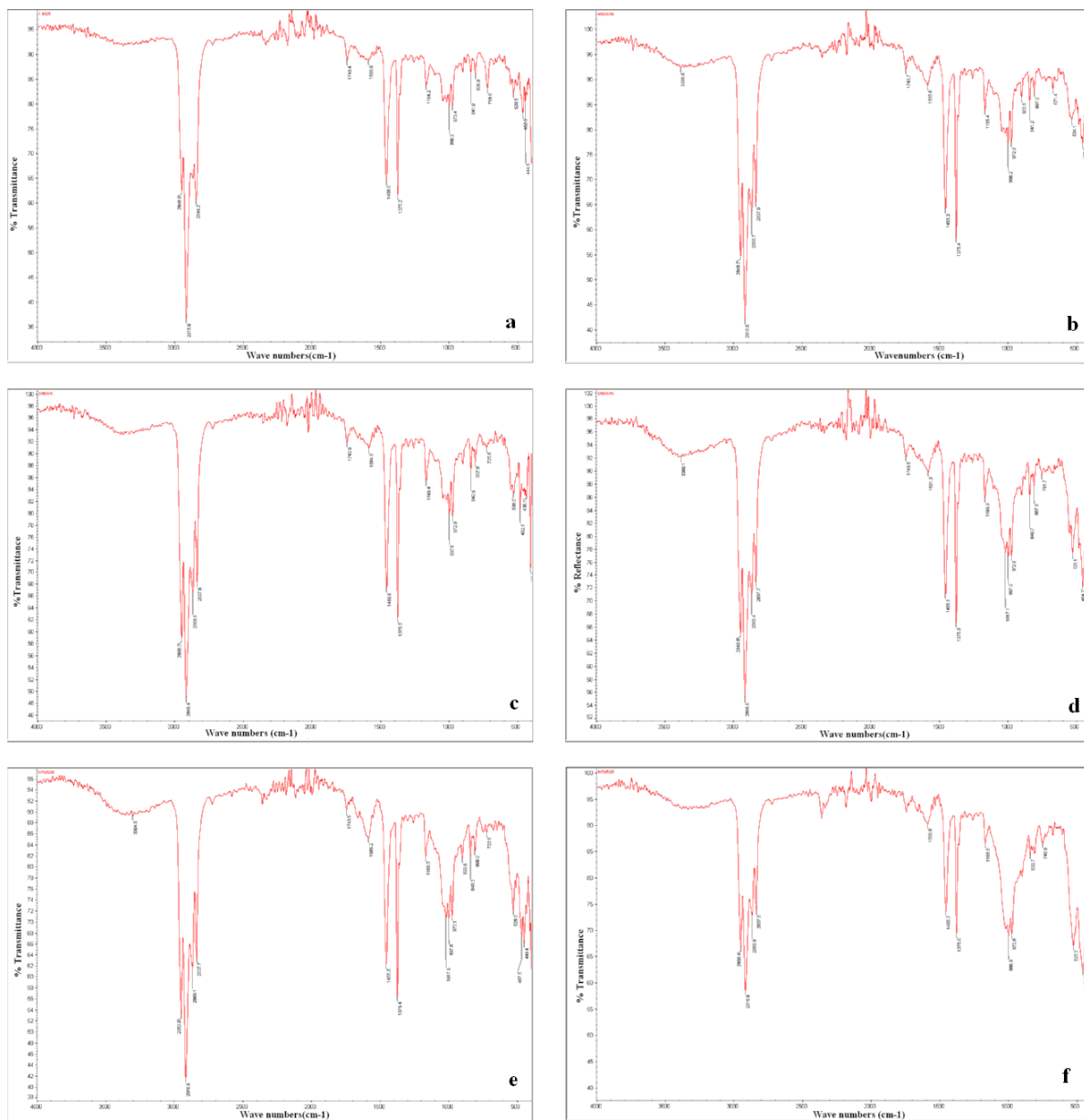
Fig. 9: FTIR Spectral data of Nanocomposites containing 5 wt%, 8 wt%, 10 wt%, 20 wt% and 25 wt% addition of Mica silicate respectively.
