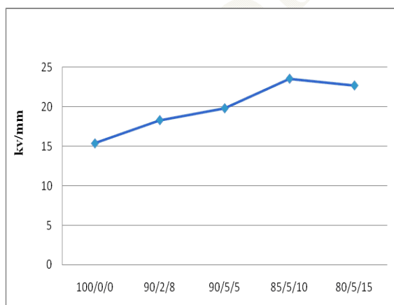
Fig. 7: Dielectric Strength
