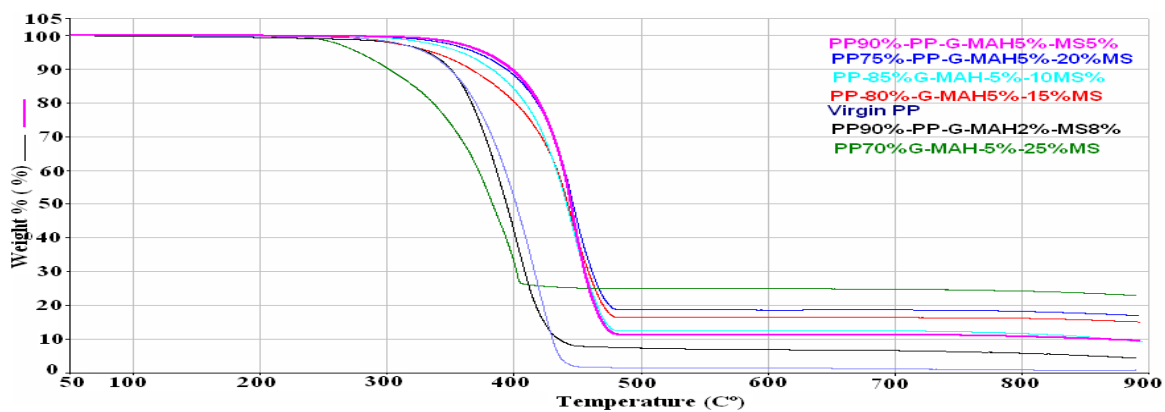
Fig. 2: TGA Curve for PP / PP - g-MAH / Mica silicate Nanoclay Nanocomposites with various compositions
