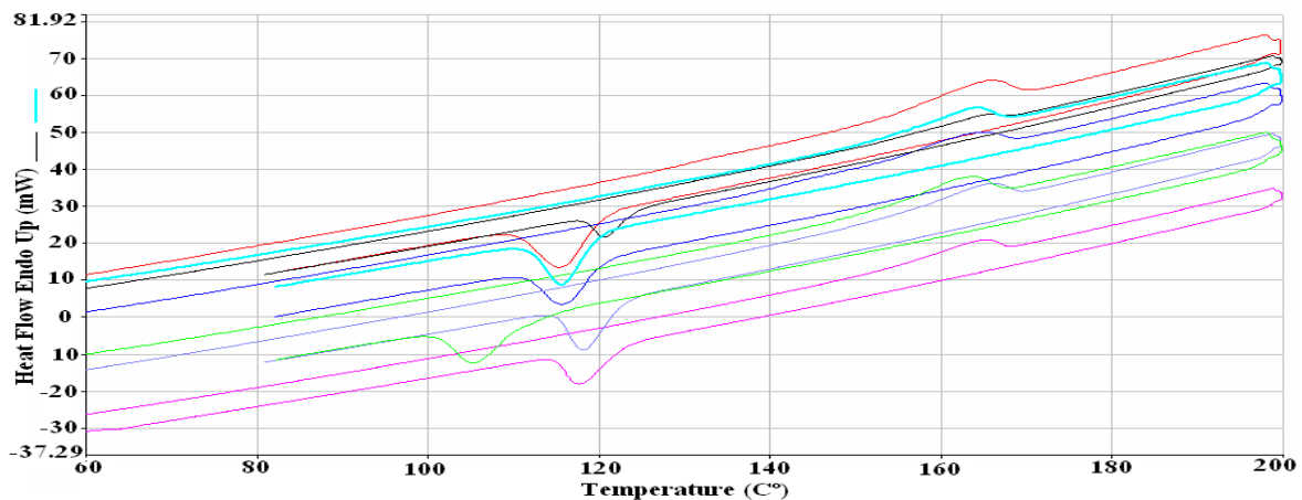
Fig. 1: DSC Curve for PP / PP - g-MAH / Mica silicate composites with various compositions
