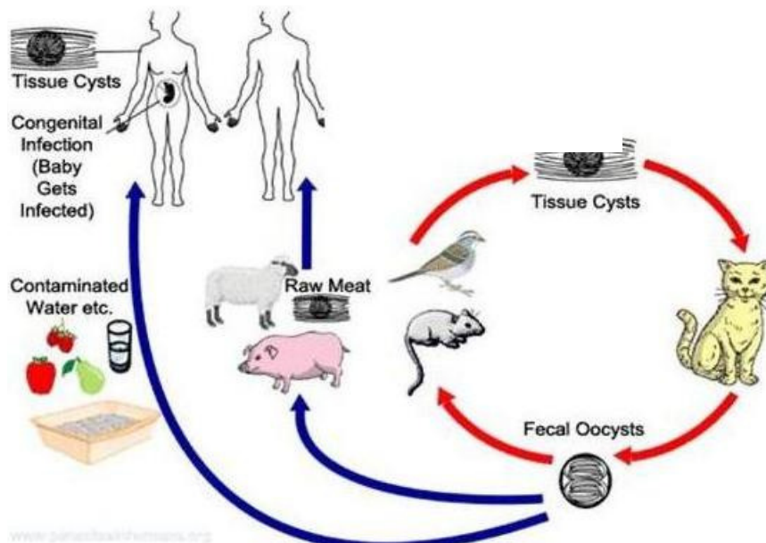
Figure 3. Life cycles of Toxoplasma gondii ( www.parasitesinhumans.org )
