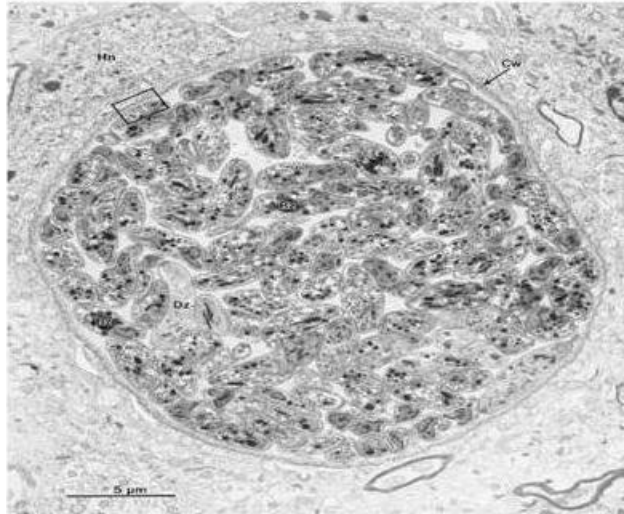
Figure 2. Electronmicrograph of tissue cyst of T. gondii containing bradyzoites (Dubey et al. , 2010)
