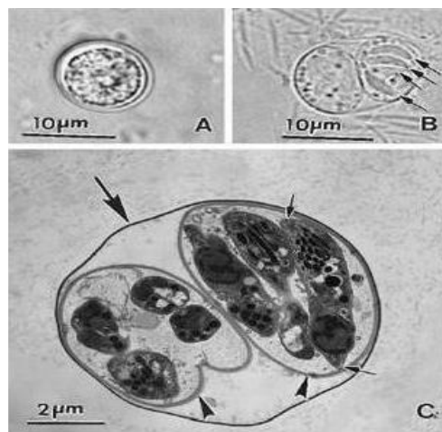
Figure 1. Oocysts of T. gondii : A = unsporulated oocysts, B and C = sporulated oocysts (arrows) (Dubey et al. , 1998).
